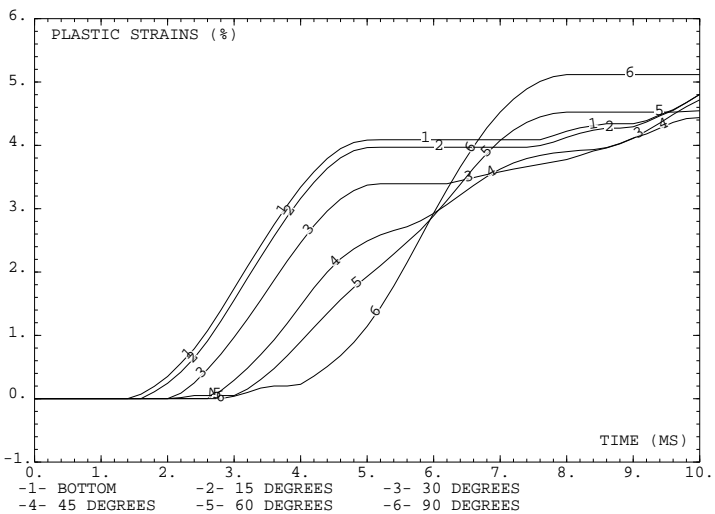
FIGURE 17: PLASTIC STRAINS ALONG THE SHELL, FROM THE BOTTOM
