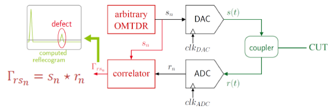
Fig. 4. Schematic diagram of wiring diagnosis based on OMTDR technology. From [111].
