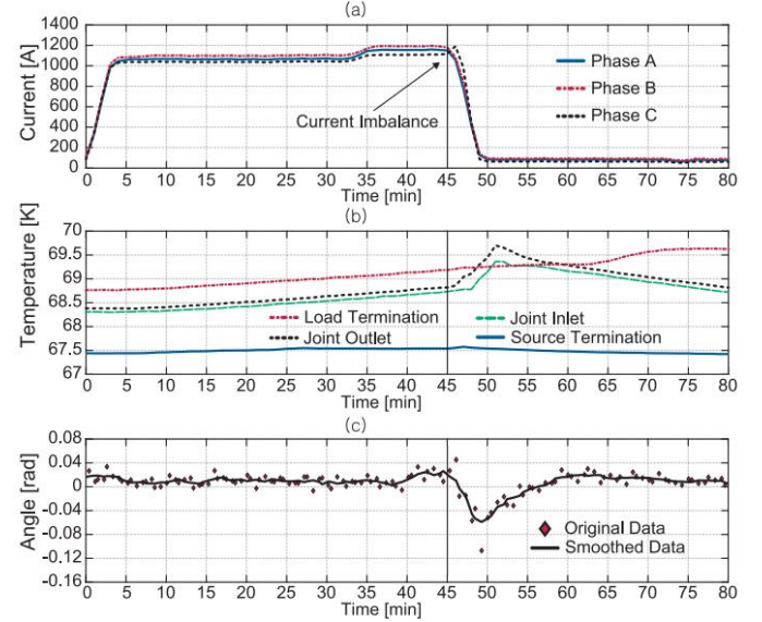
Fig. 14. Results of the current imbalance induction test. (a) Current profile. (b) Temperature profile. (c) Time-frequency phase spectrum at the joint box. From [100].
