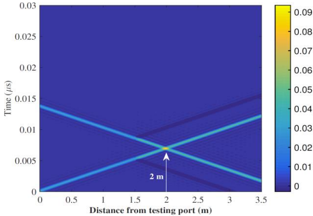
Fig. 15. A space-time ZT diagram of a single Y-junction network showing the voltage propagation after applying DORT method where a focal spot can be on the position of the soft fault. From [159].
