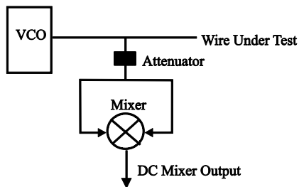
Fig. 11. MSR Circuit Diagram. From [136].
