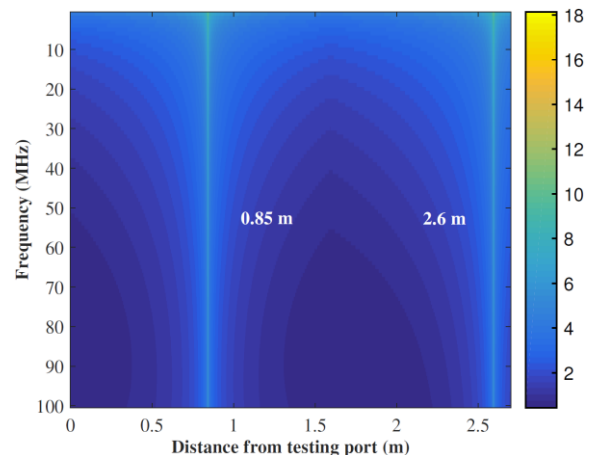
Fig. 16. Pseudo-spectrum of a single Y-junction NUT containing two soft faults, after applying the TR-MUSIC method on a frequency range from 1 to 100 MHz. From [170].
