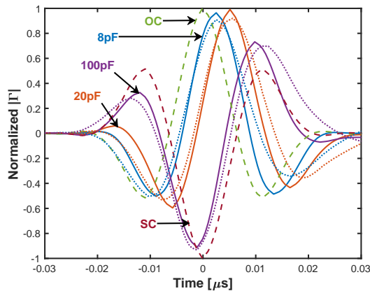
Fig. 3. SSTDR response of different capacitors connected at the end of a PV cable. From [95].
