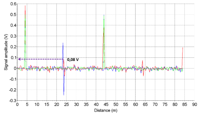
Fig. 9 Amplification of a soft defect's peak ( 1 \Omega change of a 100 \Omega line over 2 cm): Pspice model (red) and numerical model (blue) vs. standard CTDR (green). From [130].
