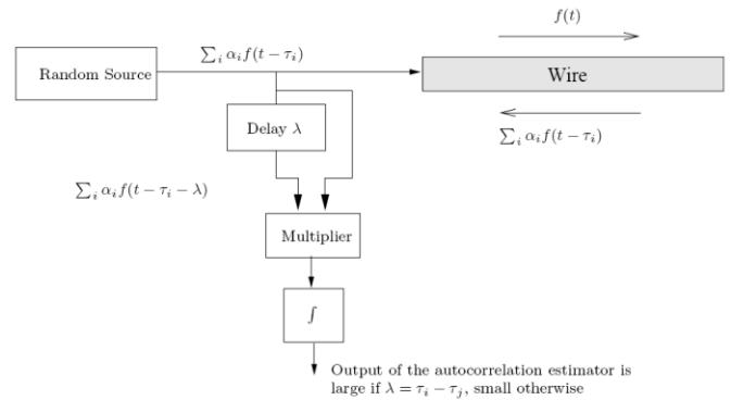
Fig. 7. NDR Type II Block Diagram. From [121].
