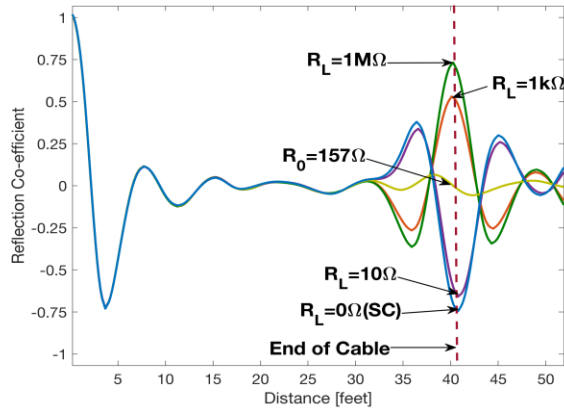
Fig. 2. SSTDR response of different resistors connected at the end of the 40-foot PV cable. The dashed red line in the figure denotes the end of the cable. From [95].
