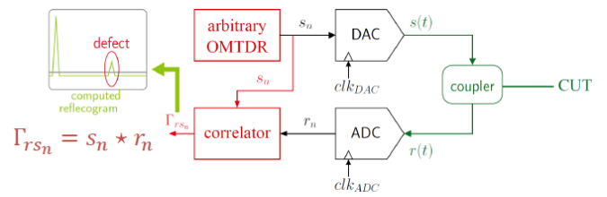
Fig. 4. Schematic diagram of wiring diagnosis based on OMTDR technology. From [111].
