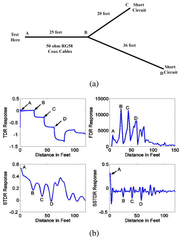
Fig. 1. (a) A network of RG-58 cables and (b) their measured responses using TDR, FDR, STDR, and SSTDR. From [85].
