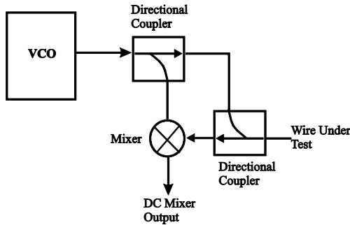
Fig. 10. PD-FDR Block Diagram. From [132].
