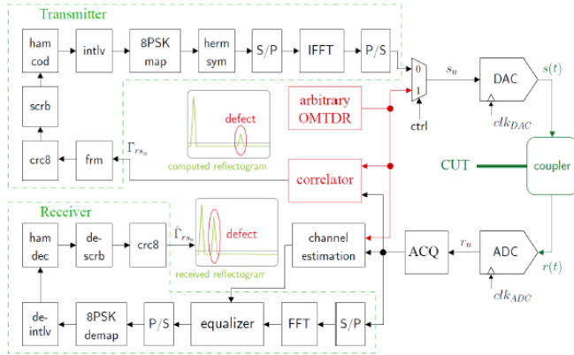
Fig. 5. A schematic diagram of sensor communication based on OMTDR technology. From [113].
