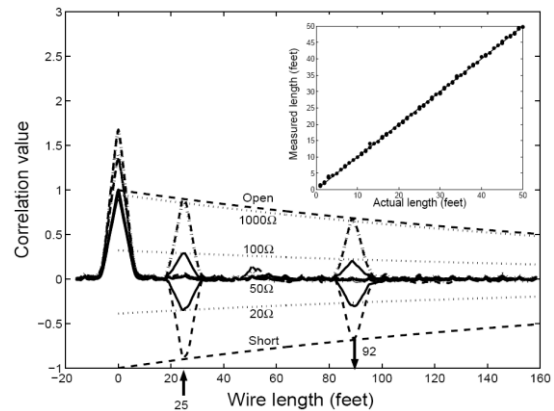
Fig. 8. Measured correlation of NDR Type II for 25 and 92 foot RG-58 (50 \Omega ) wires with resistive terminations. The inset shows the measured vs. actual length measured using an open circuited 18-gauge paired wire. This shows excellent linearity between the peak location and wire lengths. From [121].
