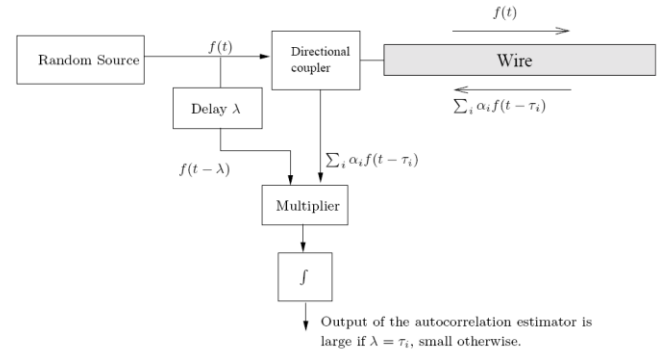
Fig. 6. NDR Type I Block Diagram. From [121].
