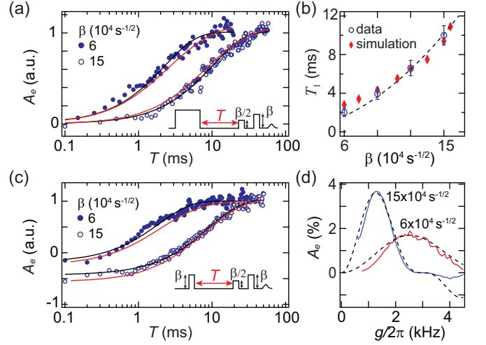
FIG. 5. Spin relaxation versus excitation amplitude (device 1). (a) Relaxation of the echo area A_e(T) as a function of the waiting time T in a saturation recovery sequence (shown in inset), for two different values of \beta . Circles and red lines correspond to measurements and numerical simulations. Black lines correspond to least square fits of the data by single-exponentials. (b) Comparison of experimentally extracted T_1 values (open blue circles) with simulated ones (red diamonds), for more \beta values. The dashed line is a quadratic fit to the data. (c) Spin relaxation measurements using inversion recovery method. (d) Calculated contribution (solid lines) of spin packets with coupling g to the echo amplitude A_e(T = 30 \text{ ms}) , for the saturation recovery sequence and the two \beta values of a). Dashed lines represent the corresponding f(\psi) function introduced in the model section.
