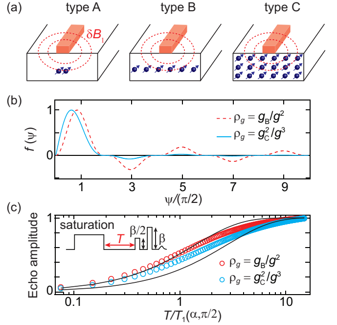
FIG. 2. Rabi angle selectivity in the narrow line case. (a) Types of spin implantation in the substrate, type A: point distribution, type B: thin layer distribution, type C: bulk distribution. Contours of rf magnetic field B_1 created by the inductor are sketched as dashed curves. (b) Calculated relative echo contribution f(\psi) from spin packets with different Rabi angle \psi . (c) Saturation recovery of the echo amplitude calculated using the model. We have taken small Rabi angles 0 < \psi < \pi . Solid black curves show exponential recovery of polarization with a decay constant T_1(\alpha, \psi_0) , where \psi_0 is the value where f(\psi) is maximum in panel (b).
