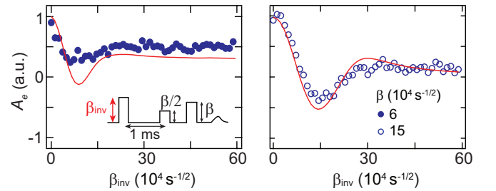
FIG. 6. Rabi oscillations measured (circles) for two different values of pulse amplitude \beta (see sequence in inset), using device 1. The fit to the data of simulations (solid red lines) provides a calibration of \beta .
