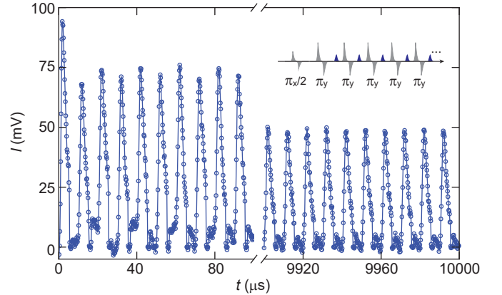
Figure 5: Averaged CPMG sequence with minimal pulse separation using bump pulses. The \pi pulses are not visible as they are being canceled by phase cycling.
