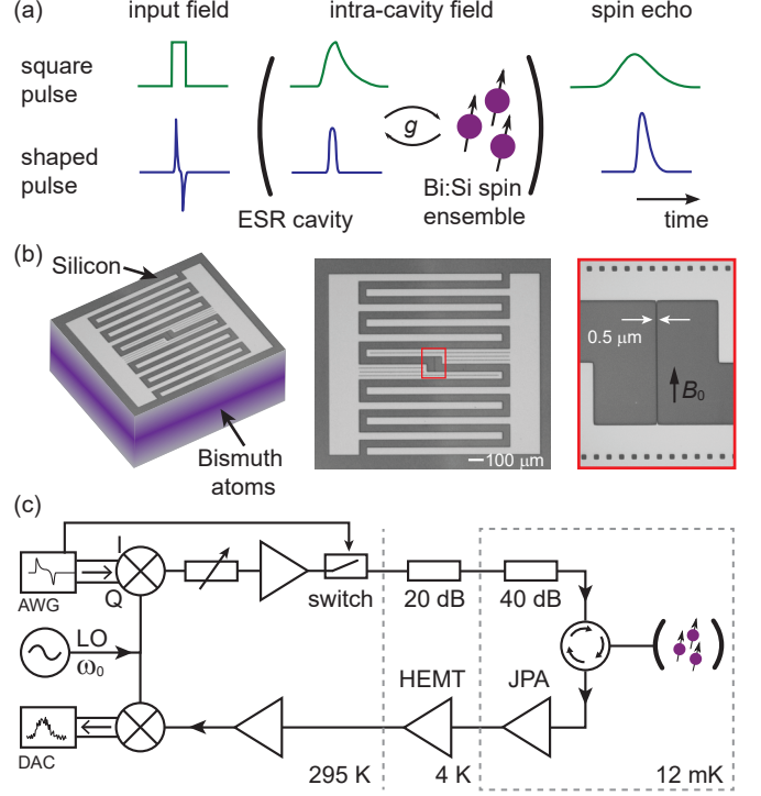
Figure 1: (a) Basic concept. A short microwave pulse with a rectangular envelope (left green line) is sent onto an ESR cavity and is subsequently distorted by the cavity's transfer function. The resulting intracavity field (center green line) then drives the spins for much longer than intended resulting in spin-echo signals which are stretched in time (right green line). In contrast, if a tailored shaped pulse is employed (left blue line), the cavity distortion is compensated. A short intracavity field (center blue line) now drives the spins resulting in wide-band spin manipulation and shorter echo duration. (b) Schematics and optical images of the LC resonator used in the experiment. Dark areas represent the Si substrate while light areas are made of Al. Bi spins are implanted everywhere below the Si surface, in a box-like profile at a depth \sim 100\text{ nm} . The resonator active area is a 0.2\text{ pL} volume around the 100\mu\text{m} -long, 500\text{ nm} -wide inductance. (c) Technical implementation. Shaped drive pulses are generated by modulating the output of a continuous-wave microwave generator (LO) by two analog outputs of an AWG via an IQ mixer. A rapid microwave switch makes sure that the sample is protected from the noise at the amplifier except when the pulses are on. The input line is strongly attenuated at low-temperatures in order to thermalize the microwave field to millikelvin temperature. The pulses are routed to the sample via a circulator, and the reflected signal is routed to the output line. It then undergoes amplification at several stages, starting from a JPA at 12\text{ mK} , followed by a HEMT at 4\text{ K} and then at room-temperature. The signal is finally demodulated using an IQ mixer, and its two quadratures digitized.
