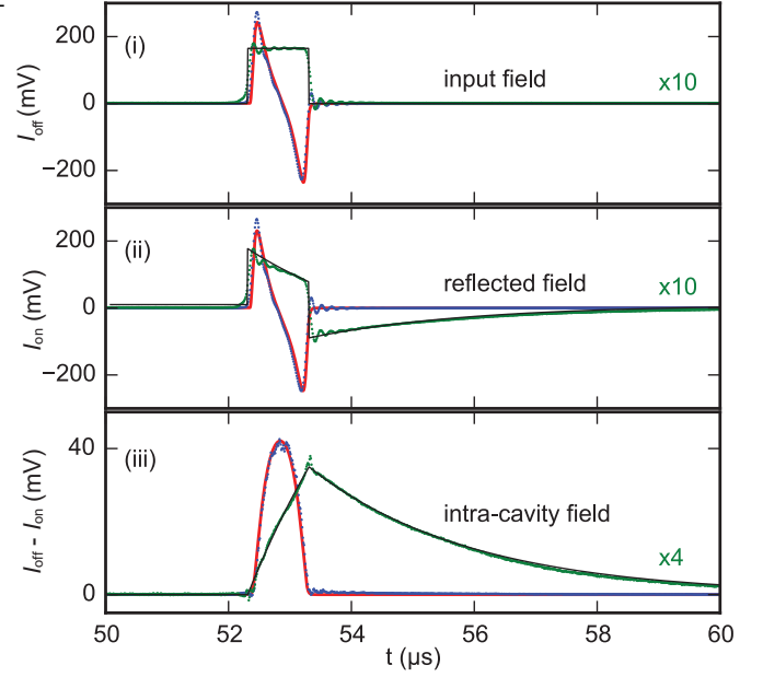
Figure 2: Reflected quadrature signal of a square (green dots) and bump-shaped (blue dots) pulses, measured 10 MHz off-resonance (i) and on-resonance with \omega_0 (ii). Subtraction yields the intra-cavity field (iii). Solid lines are from the theory. The small oscillations probably originate from parasitic resonances in the microwave setup.
