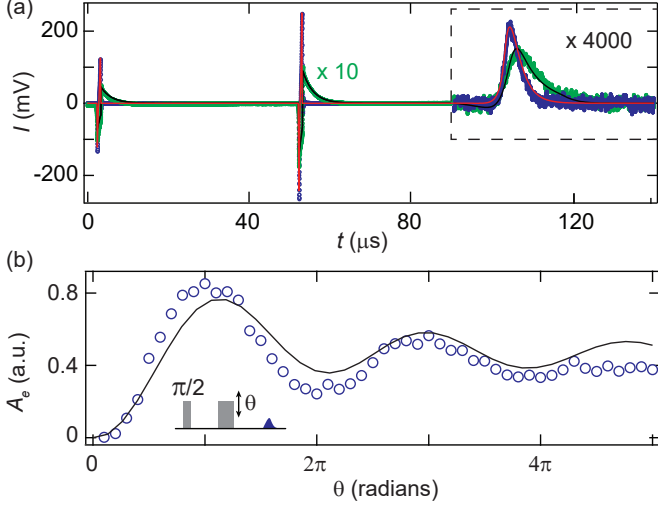
Figure 3: (a) Hahn-echo sequence with square and bump-shaped pulses. First, a \pi/2_X - \tau - \pi_Y - \tau spin-echo was measured (inset). The corresponding control pulses were sampled immediately afterwards, with only a change in amplifier gain at the detection to compensate for the larger signal amplitude. For convenience, the two control pulses were this time generated on the same quadrature, which is shown here in the main panel. Open circles are data (green for square, blue for bump), and solid lines are results from the simulation (black for square, red for bump). (b) Rabi oscillations (blue dots) and simulation (black line) for a square-shaped-pulse Hahn echo sequence with varying refocusing pulse amplitude.
