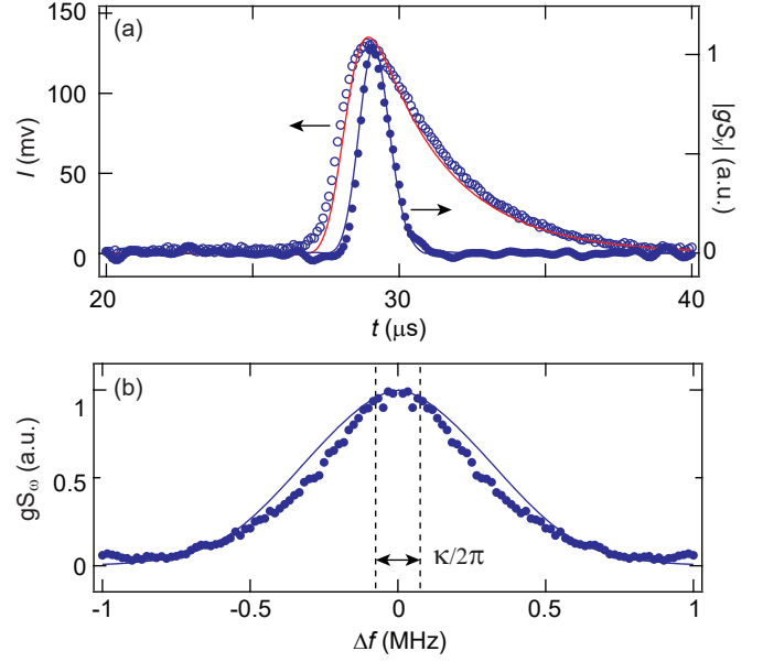
Figure 4: (a) Quadrature signal of the emitted echo (open circles) and its effective spin component gS_y obtained by de-convolution of the cavity response (filled circles). The measurement is acquired with a repetition time of t_r = 1\text{s} . (b) Fast Fourier transform of gS_y showing the spectral bandwidth of the echo, much larger than the cavity bandwidth \kappa/2\pi . Solid lines are numerical simulations.
