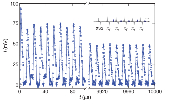
Figure 5: Averaged CPMG sequence with minimal pulse separation using bump pulses. The \pi pulses are not visible as they are being canceled by phase cycling.
