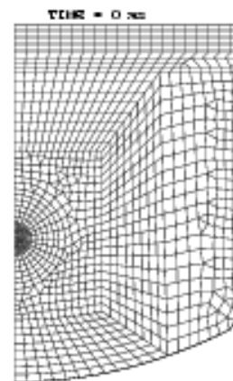
Fig. 3: Mesh of the MARAS test
