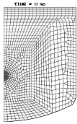
Fig. 3: Mesh of the MARAS test
