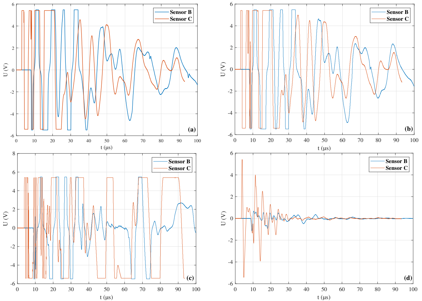
Fig. 5: Amplitude of the FOTs' voltage as measured by sensors B and C for the faults triggered by: (a) CB and 30\ \Omega resistance, (b) CB and 60\ \Omega resistance, (c) CB with the spark ignitor, and (d) CB with the spark ignitor and a 60\ \Omega resistance.
