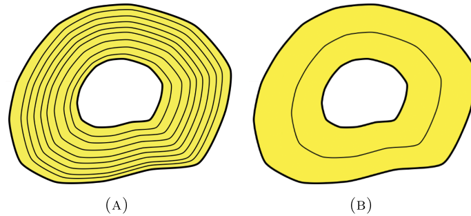
FIGURE 1. Onion-skin like domain decomposition (A) General case (B) Case of 2 subdomains.
