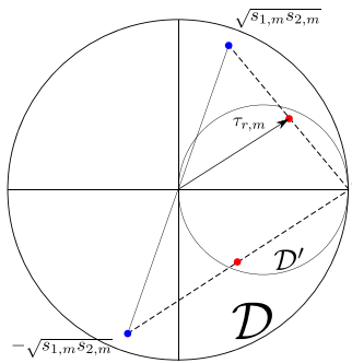
FIGURE 3. Effect of the relaxation on the eigenvalues of the unrelaxed problem (representation for r = \frac{1}{2} ). Blue dots represent the unrelaxed eigenvalues, in red are the relaxed ones.
