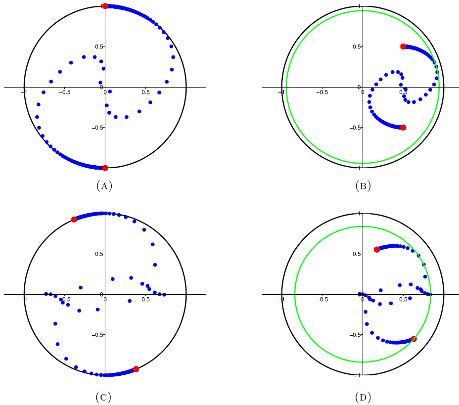
FIGURE 5. Representation in the complex plane of the unrelaxed (left) and relaxed (right) eigenvalues of A_{r,m} for the non local operator: t_m = \alpha + \beta \frac{m}{kR} . For the two plots on the top, we used \alpha = \beta = 1 , and for the two plots on the bottom we used \alpha^* = 0.31 , and \beta^* = 0.21 . Also, r^* = 0.6 . The red dots denote the limits of the eigenvalues for m \rightarrow \infty . (A) t_m = 1 + \frac{m}{kR} without relaxation (B) t_m = 1 + \frac{m}{kR} with relaxation ( r = \frac{1}{2} ) (C) t_m = \alpha^* + \beta^* \frac{m}{kR} without relaxation (D) t_m = \alpha^* + \beta^* \frac{m}{kR} with relaxation ( r = r^* ).
