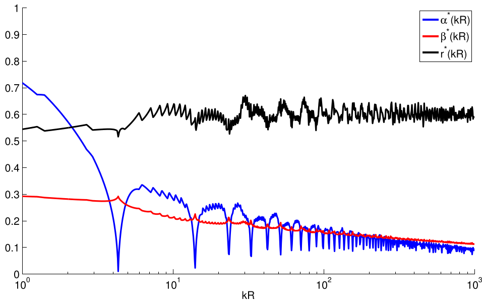
FIGURE 9. Evolution of the optimized coefficients \alpha^*(k) , \beta^*(k) and r^*(k) versus the wavenumber. kR varies from 1 to 1000.
