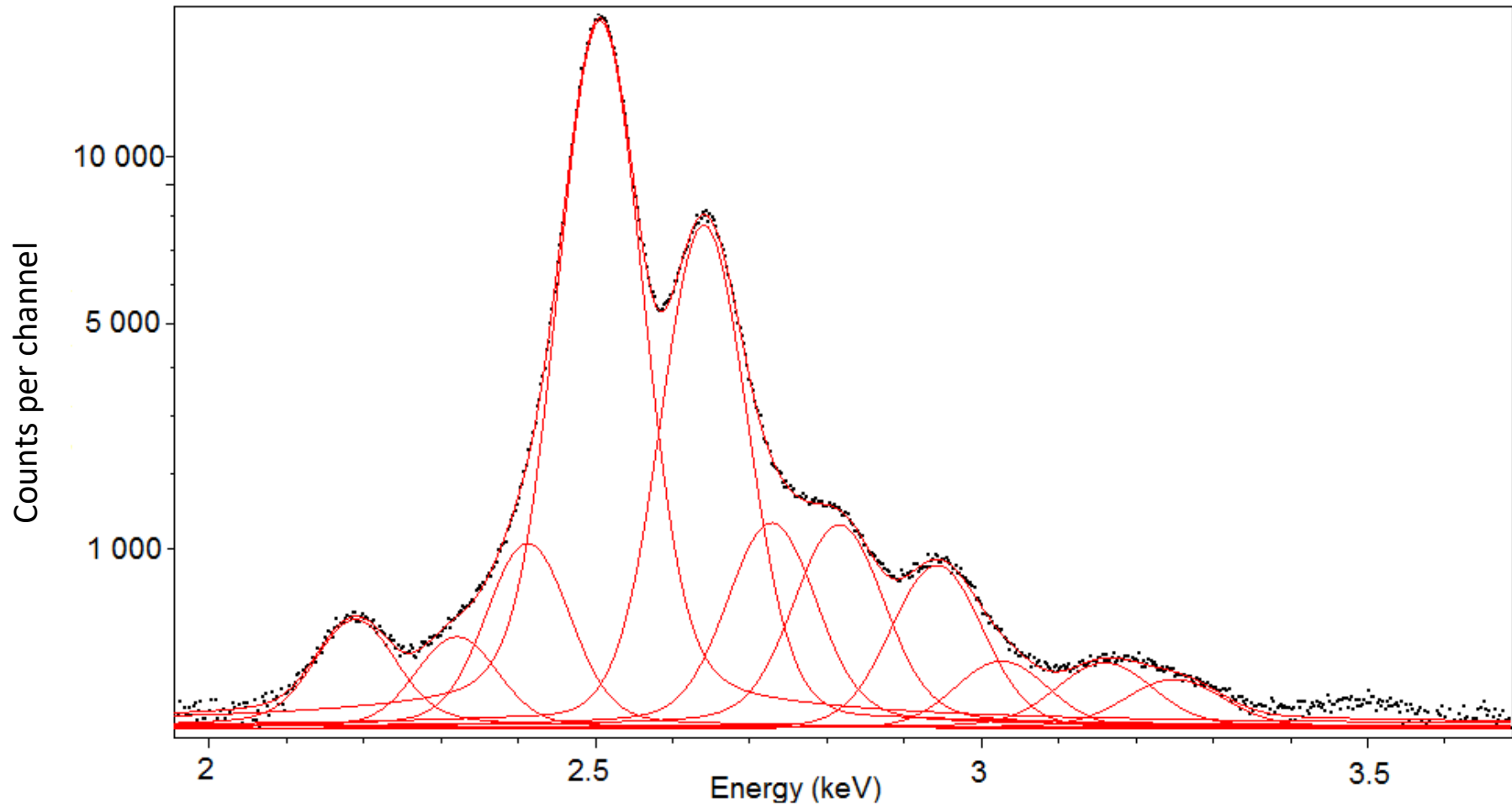
Figure 7: Processing of the Rh L X-ray region recorded by SDD detector, using Voigt functions
