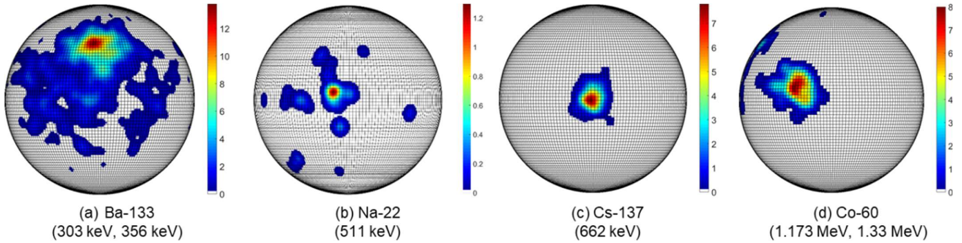
Figure 11: Compton imaging results obtained with the Timepix3 detector for different radionuclides positioned in a 2\pi sr field-of-view: (a) Ba-133, (b) Na-22, (c) Cs-137, (d) Co-60. The energy lines used to reconstruct the images are given for each radionuclide. For each measurement, the distance between the Timepix3 detector and the radioactive source is 1 m, total exposure time is 1 h.
