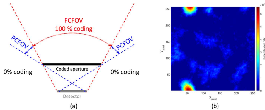
230 231 Figure 10: (a) Field-of-view and coding fraction illustration of a coded-aperture gamma camera showing the Fully Coded Field-Of-View 232 (FCFOV), and the Partially Coded Field-Of-View (PCFOV). (b) Localization of a Cs-137 source, using coded-aperture imaging, positioned at 233 the border of the fully coded field-of-view. The source is positioned in the upper part of the coded-aperture field-of-view. The distance between 234 the source and the detector is 1 m. The measurement is carried out with the MAM procedure with a total exposure time of 1 h (30 min in mask 235 mode, and 30 min in anti-mask mode). 236
