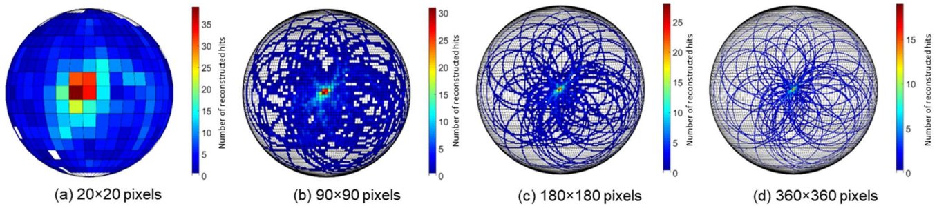
Figure 4: Impact of the half-sphere pixel grid on which are projected the Compton cones: (a) 20 \times 20 pixels; (b) 90 \times 90 pixels; (c) 180 \times 180 pixels; (d) 360 \times 360 pixels.
