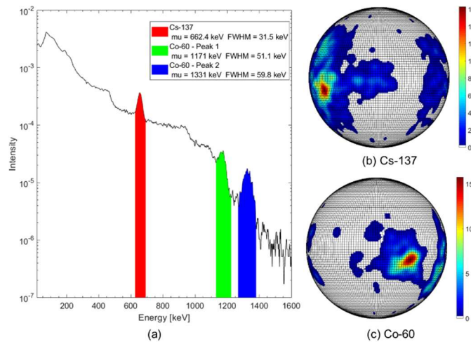
299 300 Figure 14: Multiple sources localization with Timepix3 and Compton mode (Cs-137 and Co-60 simultaneously positioned within the 301 field-of-view): (a) measured energy spectrum, with peaks used for radionuclide identification are coloured; (b) reconstructed image when 302 energy line of Cs-137 is selected; (c) reconstructed image when energy lines of Co-60 are selected.
