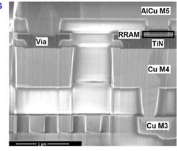
Fig. 1: Description of the process flow and SEM cross section of the integrated OxRAM
