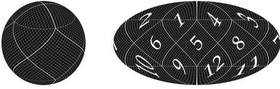
Fig. 1. HEALPix grid (visualizing N_{\text{side}} = 16 ) in orthographic projection on the left and Mollweide projection on the right . Faint lines indicate the circles of latitude \theta = \cos^{-1}(\pm \frac{2}{3}) . The right image also introduces the numbering of the faces, used in the following illustrations.
