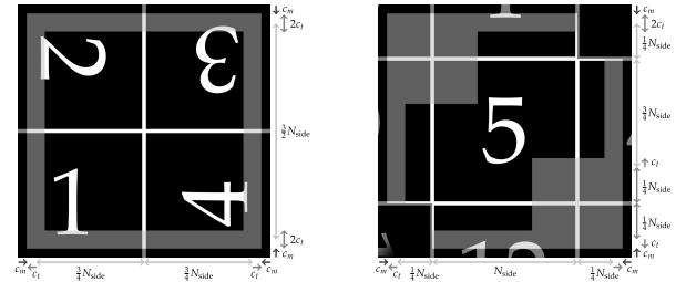
Fig. 5. Detailed view of two of the six extended faces. The dark outer boundary with width c_m is the margin that is discarded after the reconstruction step, and the two dark squares in the corners of the equatorial face on the right are treated likewise. The remaining part of the extended faces has a gray outer boundary of width 2c_t . In conjunction with the gray squares in the corners of the equatorial face, this boundary forms the transition zone that contains the values shared with the neighboring extended faces.
