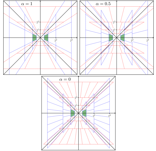
Fig. A.3. Frequency concentration of \alpha -shearlets for different values of \alpha . One sees that each “dyadic annulus” \{\xi : |\xi| \approx 2^j\} is split into a number N_j^{(\alpha)} of “wedges” representing the different directions. In fact, N_j^{(\alpha)} \approx 2^{(1-\alpha)j} .
