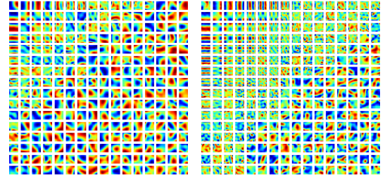
Fig. 10. Atoms learned in the multiscale dictionary learning approach: on the left , scale 3, on the right , scale 2. The dictionaries have departed from the original redundant DCT dictionary and have learned specific features related to the scale. Due to the change of the N_{\text{side}} parameter with the scale, the actual distance between two adjacent pixels has increased, and the atoms for scale 2 are indeed smoother than those for scale 3.
