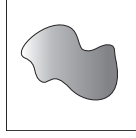
Fig. A.1. Example of a cartoon-like function. Such a function f is smooth, apart from a jump discontinuity along a curve \gamma . Even though f might be discontinuous along \gamma , the boundary curve \gamma itself is required to be smooth.
