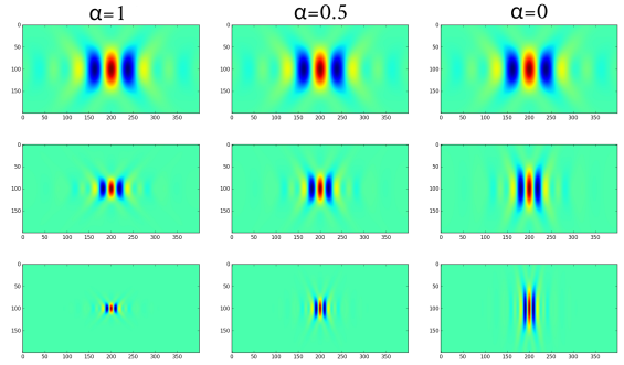
Fig. A.2. Effect of dilating a “prototype function” \psi (shown at the top of each column) with the matrices D_j^{(\alpha)} to obtain \psi(D_j^{(\alpha)} \bullet) , for different values of the scale j (going from j = 0 (top panels) to j = 2 (bottom panels)) and of the “anisotropy parameter” \alpha \in [0, 1] .
