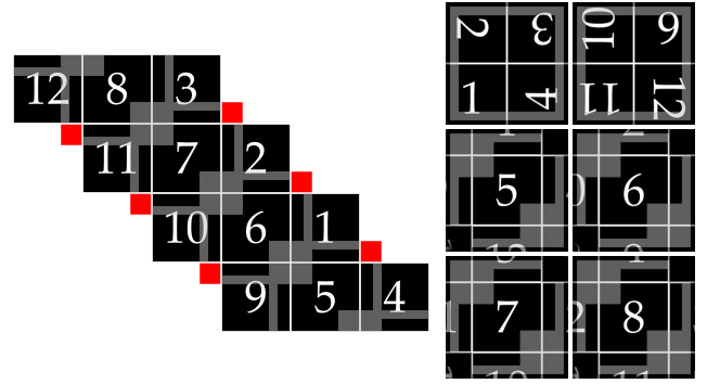
Fig. 4. Left panel: twelve squares corresponding to the faces of the HEALPix framework (see Fig. 1) arranged as a net in the plane. The areas that are covered by multiple of the extended faces – the transition zones – are displayed in gray. The areas where pixels are “missing” are displayed in red. Right panel: six extended faces produced by the patchwork procedure. The two polar faces form the top row, followed by the four equatorial faces below. The shaded area around the transition zone of each composite face indicates the margin, which is later discarded.
