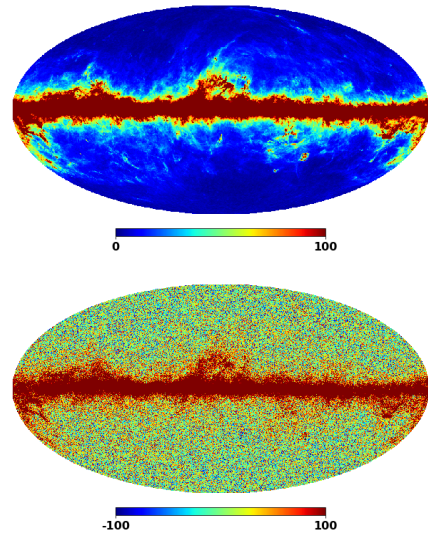
Fig. 7. Thermal dust simulation map (at 100 GHz) without (top panel) and with the additive white Gaussian noise added (bottom panel), for evaluation of the methods. The colorscale has been stretched to illustrate the challenge of recovering structures at intermediate latitude. Units are in \mu\text{K} .
