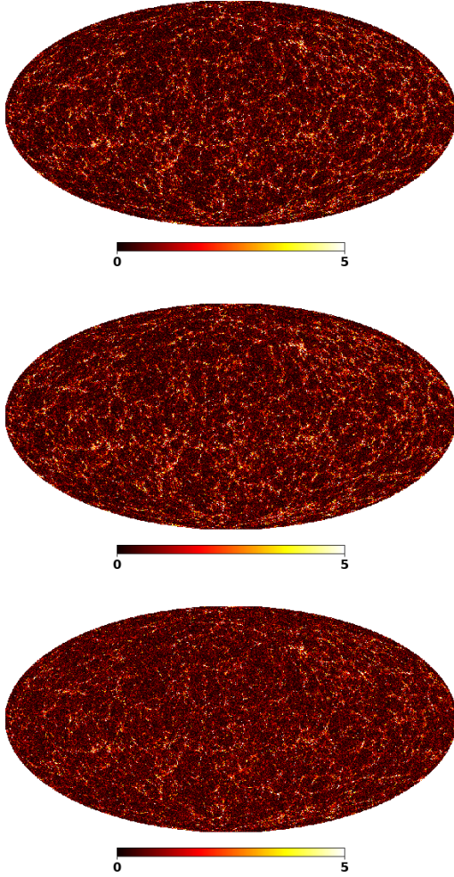
Fig. 16. Amplitude of the residuals for all three approaches, for the dark matter map scenario. Top and middle panels: \alpha -shearlet denoising with rotation-based ( top ) or patchwork ( middle ) approach, both with \alpha = 1 . Bottom panel: representation learned with dictionary learning.
