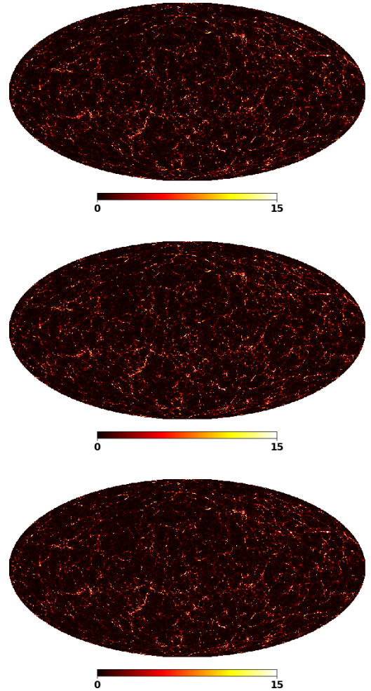
Fig. 15. Denoised dark matter maps for all three approaches. Top and middle panels: \alpha -shearlet denoising with rotation-based ( top ) or patchwork ( middle ) approach, both with \alpha = 1 . Bottom panel: representation learned with dictionary learning.
