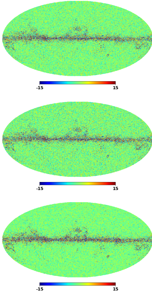
Fig. 14. Residuals for the maps displayed in Fig. 12. Units are in \mu\text{K} .
