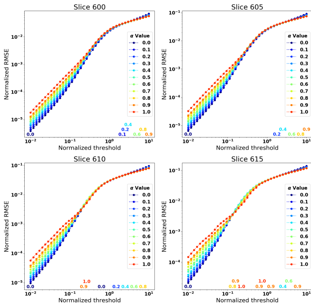
Fig. 20. Normalized non-linear log-approximation curves for four different slices of the dark matter distribution. For each threshold, the \alpha value corresponding to the lowest approximation error is displayed on the bottom.
