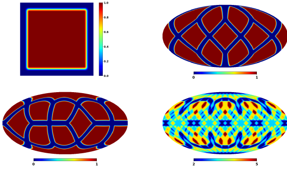
Fig. 3. Partition of unity for the rotation-based reconstruction. The weights smoothly decaying toward the border are presented in the top left panel and are copied to each HEALPix face in the top right panel . In the bottom left panel , resampling was first performed using a rotation and bilinear interpolation, and the image shows the weights that would be applied in the original reference coordinates. The resulting covering of the sphere using five rotations is illustrated in the bottom right panel .
