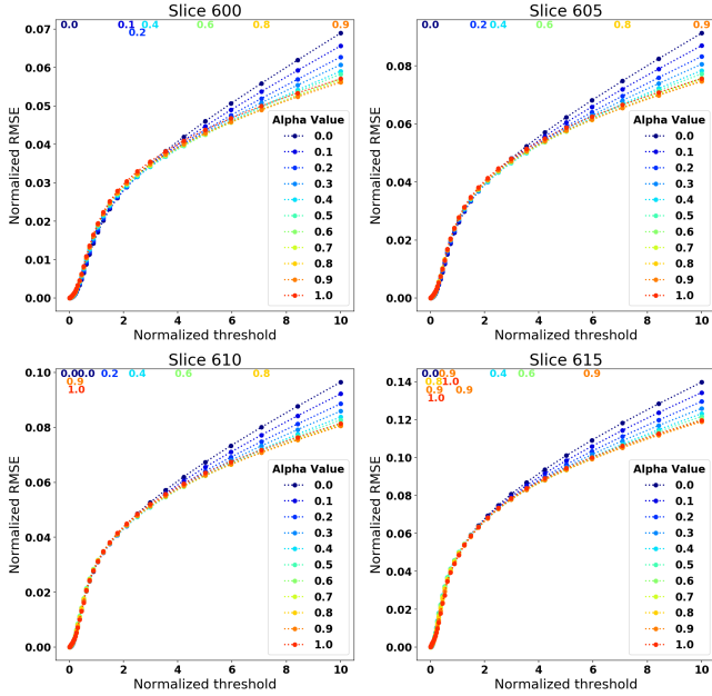
Fig. 19. Normalized non-linear approximation curves for four different slices of the dark matter distribution. For each threshold, the \alpha value corresponding to the lowest approximation error is displayed on the top.
