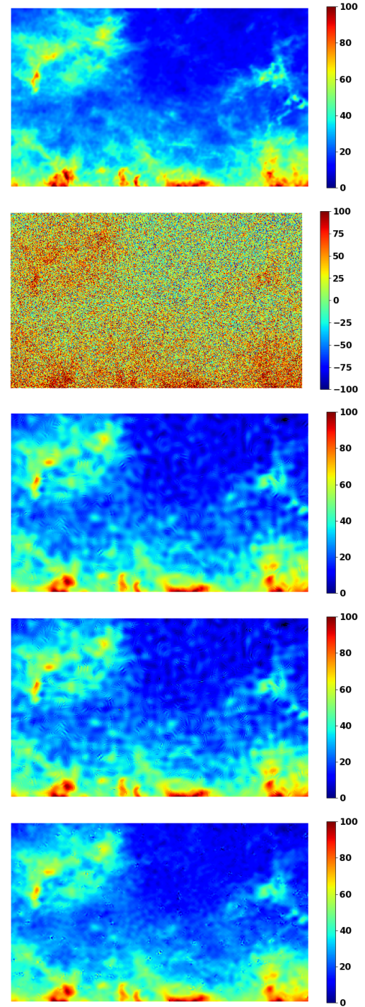
Fig. 13. Zoom on a region close to the galactic plane to visualize the respective denoising performance of the methods. From top to bottom panels: input map, noisy map (with own colorscale), rotation-based approach with \alpha = 0.6 , patchwork approach with \alpha = 0.6 , sparse representation learned from data. All units are in \mu\text{K} .
