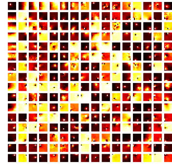
Fig. 11. Atoms learned in the dictionary learning approach, applied to the dark matter halo distribution data. The dictionary elements are composed of point-like structures and edges.
