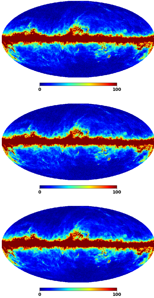
Fig. 12. Denoised thermal dust maps for all three approaches. Top and middle panels: \alpha -shearlet denoising with rotation-based ( top ) or patchwork ( middle ) approach, both for \alpha = 0.6 . Bottom panel: representation learned with dictionary learning. Units are in \mu\text{K} .
