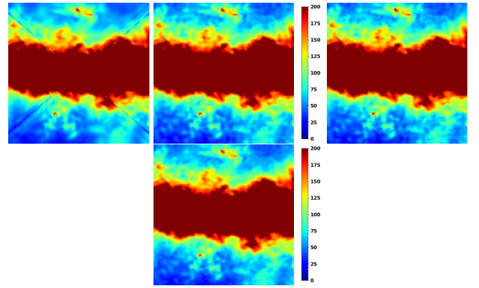
Fig. 18. Cartesian projection of the denoised thermal dust maps centered at the intersection of four faces. From left to right and top to bottom panels: denoising each face independently using \alpha -shearlets with \alpha = 1 , restoration via the rotation-based approach, patchwork approach with \alpha = 1 , dictionary learning with patch width of 12. The colorscale has been stretched to visualize the artifacts seen as a cross-shape discontinuity at the boundaries of the four HEALPix faces in the upper left panel . All of our proposed approaches are free from these artifacts. Units are in \mu\text{K} .
