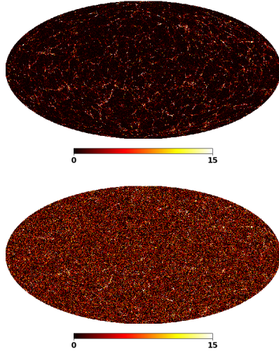
Fig. 9. Dark matter halo distribution for the first slice, without ( top panel ) and with the additive white Gaussian noise added ( bottom panel ), for evaluation of the methods. The colorscale has been stretched to visualize filamentary structures.
