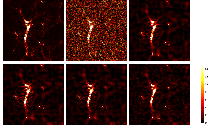
Fig. 17. Dark matter map amplitudes for all three approaches in a zoomed region. From top to bottom and left to right panels: original map, noisy map, rotation-based approach with \alpha = 1 , patchwork approach with \alpha = 0 , patchwork approach with \alpha = 1 , representation learned from data.
