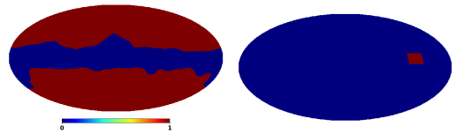
Fig. 8. Left panel: galactic mask used for thermal dust quantitative evaluation, covering 70% of the sky. Right panel: region close to galactic plane where methods are inspected.
