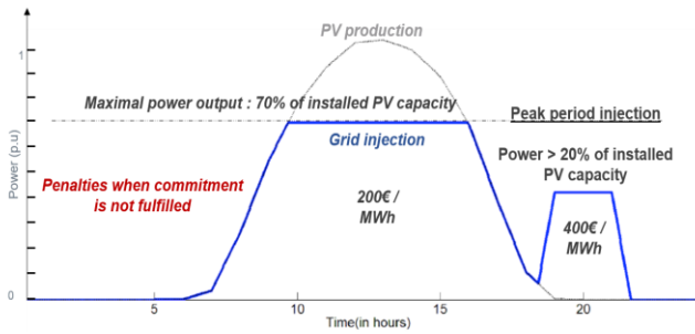
Fig. 2. Application #1 - Daily injection profile (illustration)
