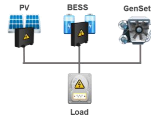
Fig. 5. application #2 - Hybrid microgrid topology
