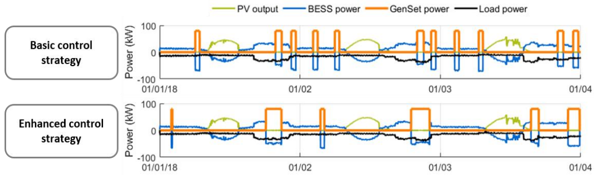
Fig. 8. Comparison of simulated operation with different control strategies
