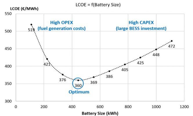
Fig. 7. application #2 - Optimal sizing baseline
