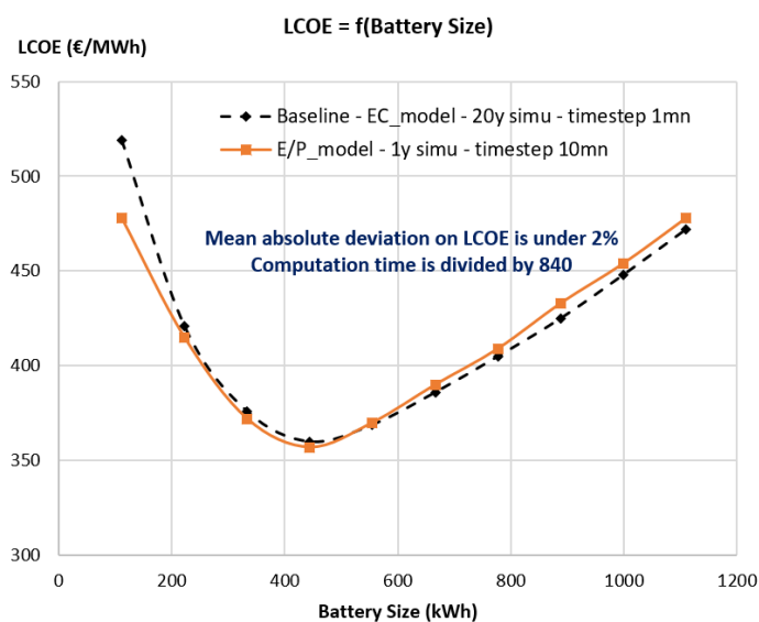
Fig. 11. Conclusive approximation with a time reduction factor of 840
