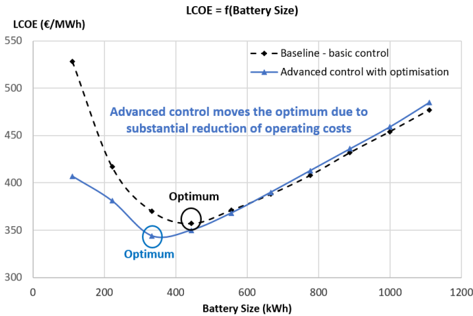
Fig. 9. Influence of control strategy on optimal size determination
