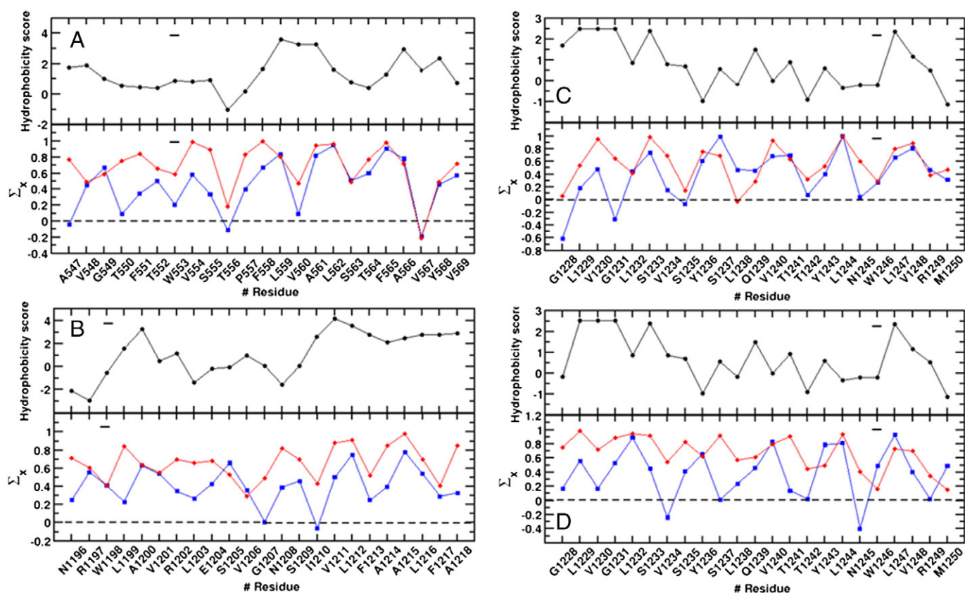
Fig. 10. Differences in SASA_x and hydropathicity for the (A) mTM10, (B) mTM16, (C) TM17 and (D) KTM17 peptides. In each panel, the hydropathicity scale and the relative difference in SASA_x between the water and the micelle environment is presented in the upper and lower part respectively. The hydropathicity scale of each residue (black) was computed with the Kyte–Doolittle approach [103] used by the ExPASy server [104] with a window of three. Regions with values above and below zero are considered as hydrophobic and hydrophilic, respectively (see main text for details). In the panels, results for DPC are in blue and in red for DDM. The black line in the figures highlights the tryptophan residue positions of each peptide.
