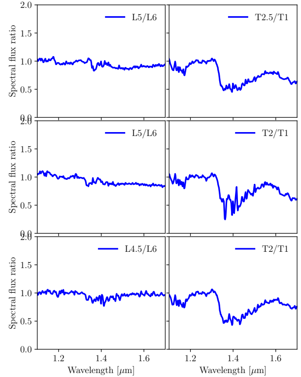
Fig. 1. Left: spectral-flux ratio of the L5 dwarf 2MASS J01550354+0950003, L5 2MASSW J1507476-162738, L4.5 SDSS J083506.16+195304.4 to a reference L6 dwarf 2MASSI J1010148-040649. Right: spectral-flux ratio of the T2.5 dwarf IPMS J013656.57+093347.3, T2 2MASS J11220826-3512363, T2 SDSSp J125453.90-012247.4, to a reference T1 dwarf SDSS J085834.42+325627.7. The data are SpeX prism spectra coming from the SpeX Prism Library (Burgasser 2014) and are similar to spectral standards.
