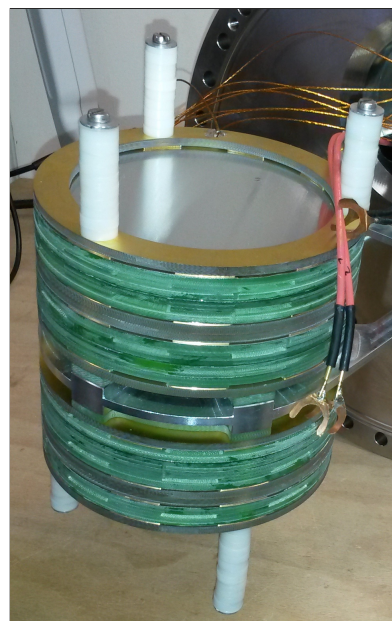
Figure 4. An example of a stack of micromegas detectors on a mounting structure for insertion in a reaction chamber.
