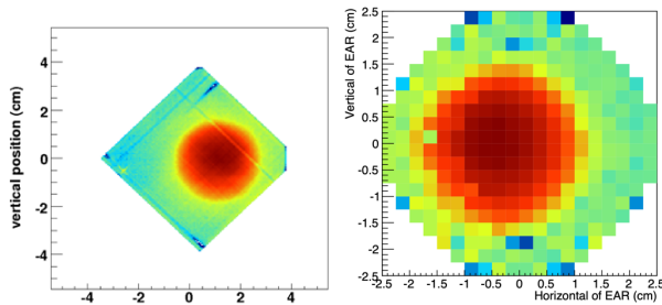
Figure 5. Neutron beam images obtained using a MicroMegas detector with XY strips (left panel). and with a pixellized MicroMegas. Figures are from ref. [18].
