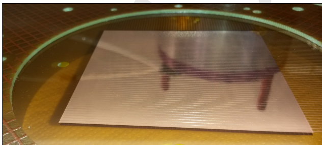
Figure 6. One side of a double sided segmented microbulk, showing the 1 mm wide strips, used for precise neutron beam imaging as function of neutron energy [20].
