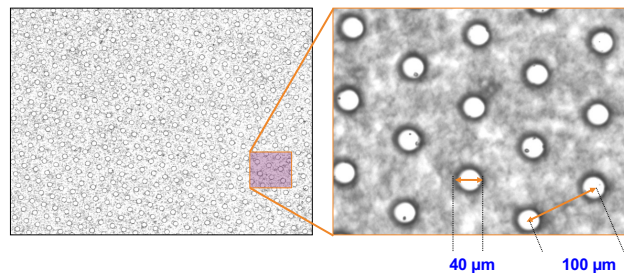
Figure 2. A microscope picture of the mesh of a microbulk detector. The patterns of the holes are clearly visible. The pitch value of 100 \mu\text{m} and the hole diameter of 40 \mu\text{m} are typical for microbulk detectors but may vary between generations and also depend on the kapton thickness and segmentation structure.
