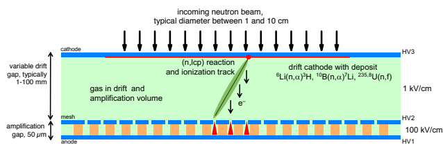
Figure 1. The principle of the microbulk MicroMegas detector as a neutron detector. The neutron beam has typically a diameter of several cm, depending on the used collimators, the detector itself is a bit larger to cover the full neutron beam. The drift electrode is coated with a thin layer of material creating charged particles by neutron-induced reactions. The resulting charged particle ionizes the gas in the drift region. The electrons are multiplied in the amplification region consisting of a chemically etched copper-coated kapton foil. The fast signal is usually read out at either the mesh or the anode.
