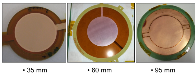
Figure 3. Three formats of single pad MicroMegas detectors with diameters of 35, 60 and 95 mm, as used in n_TOF experiments.
