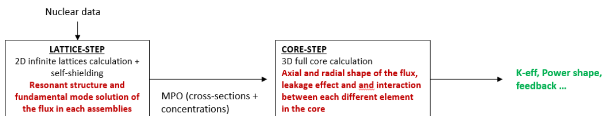
Figure 3. 2-step neutronic scheme principle.
