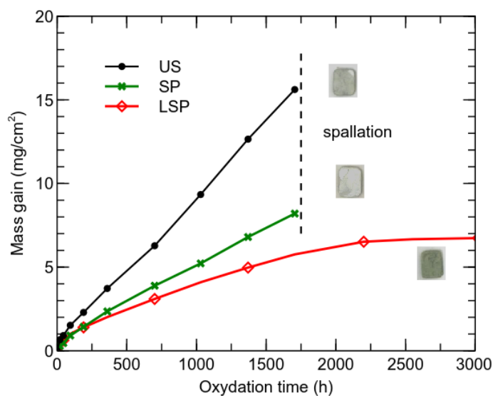
Figure 2- Mass gain as a function of the time up to 3000 h for US, SP and LSP samples at 700 °C under dry air.
