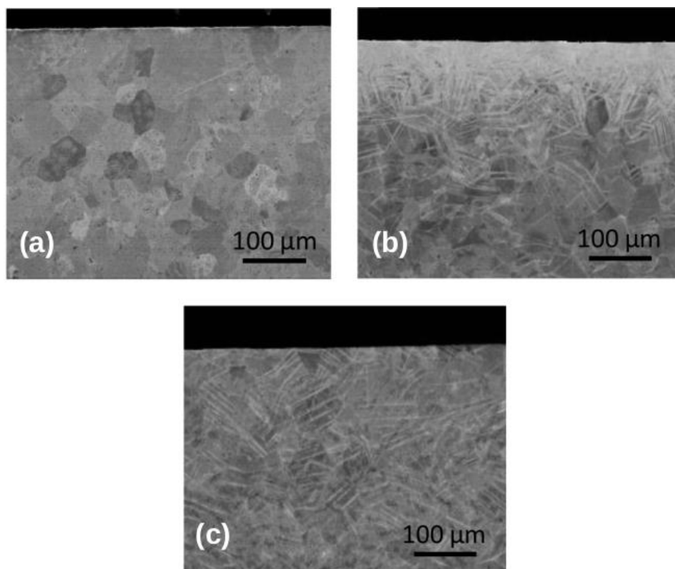
Figure 1 - Cross-section SEM images of (a) US, (b) SP and (c) LSP samples before exposition to high temperature.
