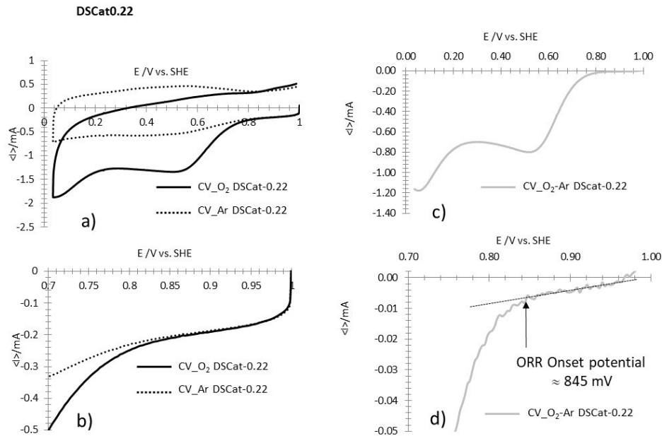
Figure A2. Example of determination of ORR onset potential for DSCat-0.22. (a) CVs recorded at 5mV·s -1 in O 2 saturated HClO 4 1M (CV O 2 DSCat-0.22) and in Argon saturated HClO 4 1M (CV Ar DSCat-0.22). (b) Enlargement of a) in the potential region of the ORR onset potential. (c) CV resulting from the difference between CV O 2 DSCat-0.22 and CV Ar DSCat-0.22. (d) Enlargement of c) in the potential region of the ORR onset potential, showing its determination (vertical arrow).
