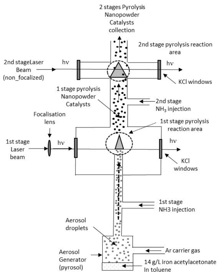
Figure 1. Scheme of the experimental set-up for two-stage ammonia-induced CO 2 laser pyrolysis.
