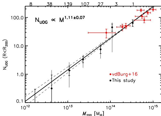
Fig. 3. Abundance of UDGs as a function of halo mass. Thick black points: averages in bins of halo mass. Two types of error are shown: thick errors with hats are Poisson uncertainties, while thin errors show bootstrap errors after resampling the groups in each bin. Thick red points: values measured for eight individual clusters in vdB16. Black lines: best-fitting power-law relation including all data points shown here. Dashes: relations corresponding to the \pm 1\sigma uncertainties on the power-law index. The numbers on the top axis indicate the number of groups in each bin.
