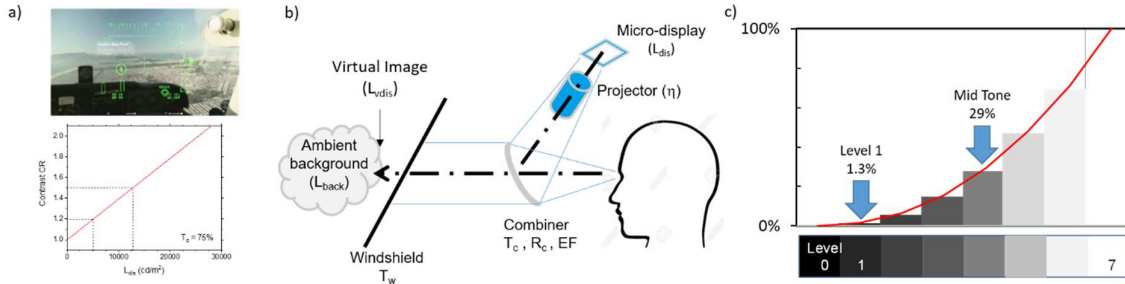
Figure 1: a) Typical scene observed by the HMD user with superposed virtual displayed image and dependence of virtual image contrast versus L_{vdis} assuming L_{back}=34,000 \text{ cd/m}^2 and T_c=75\% , b) Principle of an AR headset for avionics application; c) Grey scale and gamma curve (red).
