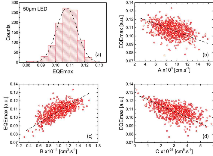
Figure 5. 1000 run Monte Carlo simulation results of a 50μm width LED. (a) Histogram Gaussian like distribution of EQE_{max} . Cloud graphs in (b), (c) and (d) represent EQE_{max} versus SRH, radiative and Auger recombination related parameters A, B and C, respectively. Awaited trends of EQE_{max} are observed versus each parameter showing the robustness of our implemented statistical approach in the SPICE model.
