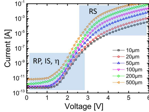
Figure 2. Current-voltage characteristics of different square LEDs. Width ranges from 10 \mu m to 500 \mu m. Shaded areas show where the SPICE model parameters, RS, RP, IS and \eta were adjusted. Note that the leakage current saturates due to a limitation in our measurement instrumentation.
