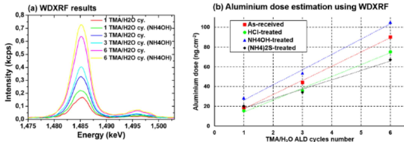
Fig. 7. (a) WDXRF Al intensities for as-received and \text{NH}_4\text{OH} -treated surfaces (b) WDXRF quantification estimation of the aluminum dose on the surfaces after 1, 3 or 6 TMA( 1^{\text{st}} )/ \text{H}_2\text{O} ALD cycles without surface treatment (as-received), with \text{HCl} , \text{NH}_4\text{OH} or (\text{NH}_4)_2\text{S} surface treatment
