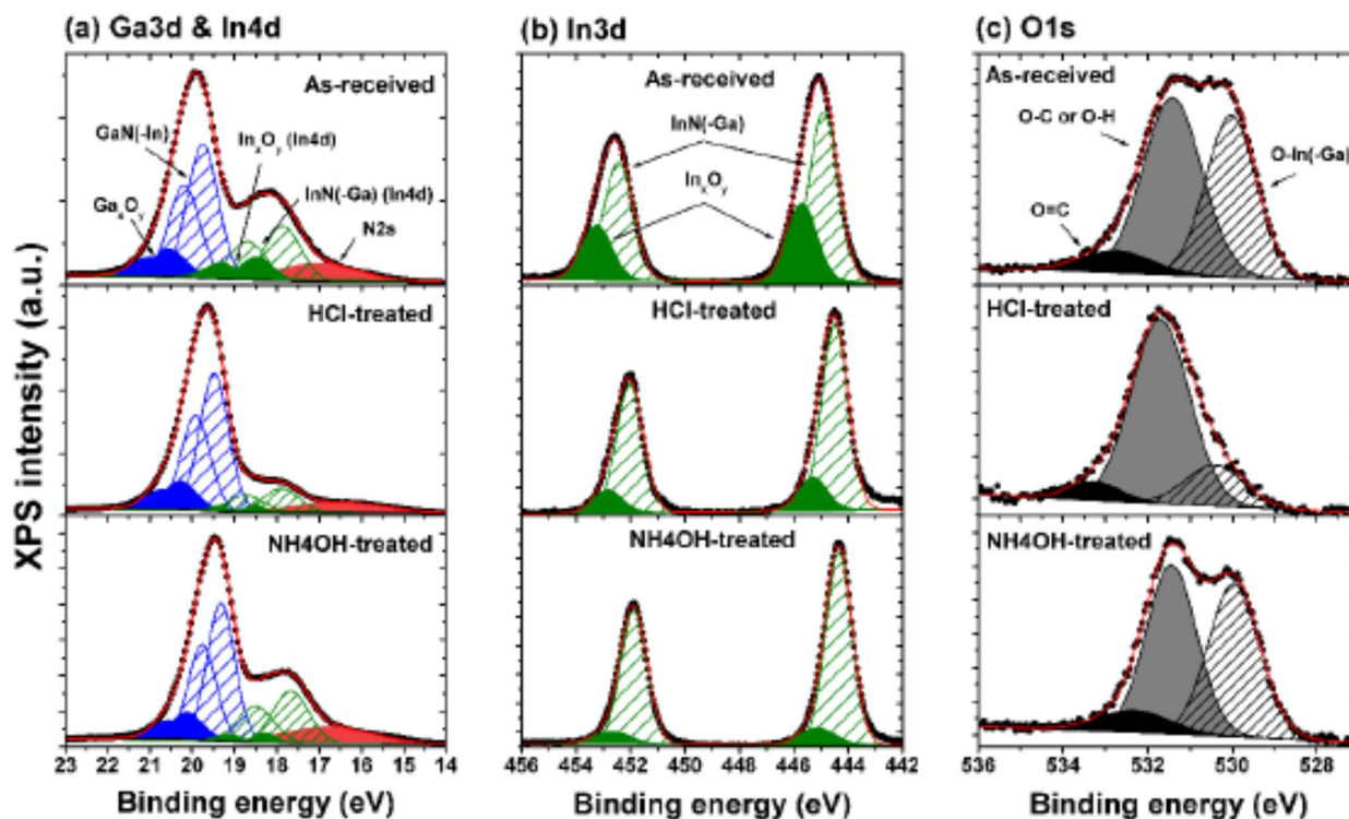
Fig. 2. Ga3d & In4d (a), In3d (b), O1s (c) spectra after HCl or NH 4 OH
