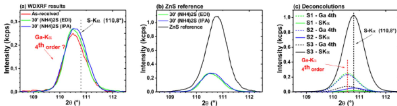
Fig. 6. (a) S K \alpha WDXRF measurements spectra of as-received sample and of 30' (NH 4 ) 2 S treated samples with EDI or IPA rinsing (b) comparison with the spectrum obtained from a ZnS/InGaN reference (c) spectra deconvolution between the Ga K \alpha 4 th diffraction order and the S K \alpha line (S1: 30' (NH 4 ) 2 S treated with EDI rinsing; S2: 30' (NH 4 ) 2 S treated with IPA rinsing; S3: ZnS reference)
