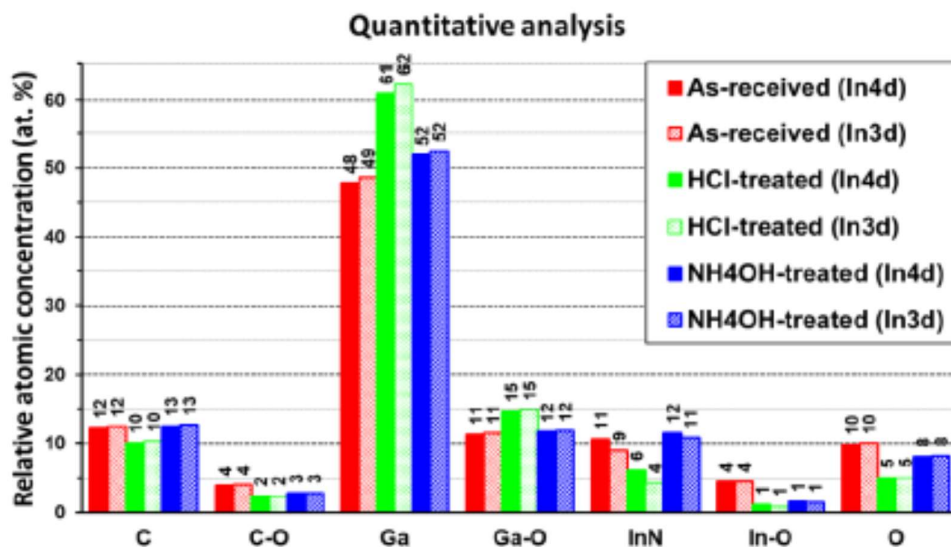
Fig. 3. Relative atomic concentrations estimated from XPS quantitative analysis of samples after HCl or NH 4 OH treatments, using In3d or In4d lines
