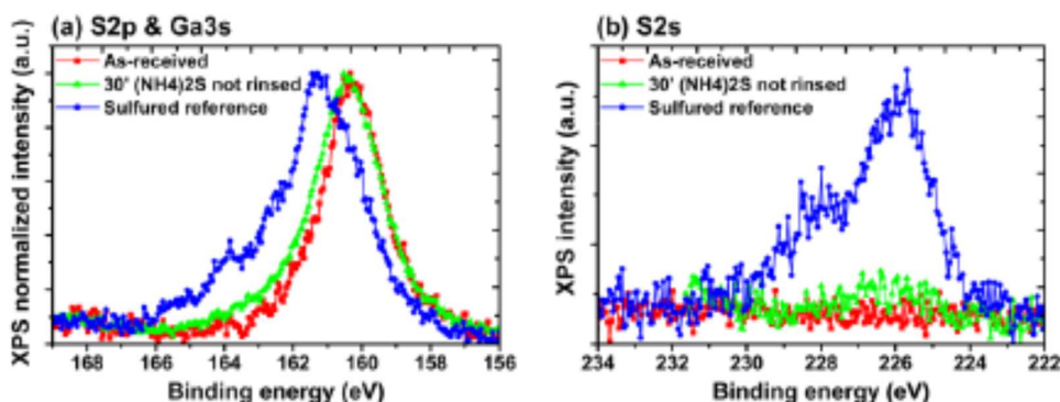
Fig. 5. (a) Superposition of S2p-Ga3s normalized XPS spectra of as-received, 30' (NH 4 ) 2 S-treated and sulfur reference samples (b) Superposition of S2s spectra of the same samples
