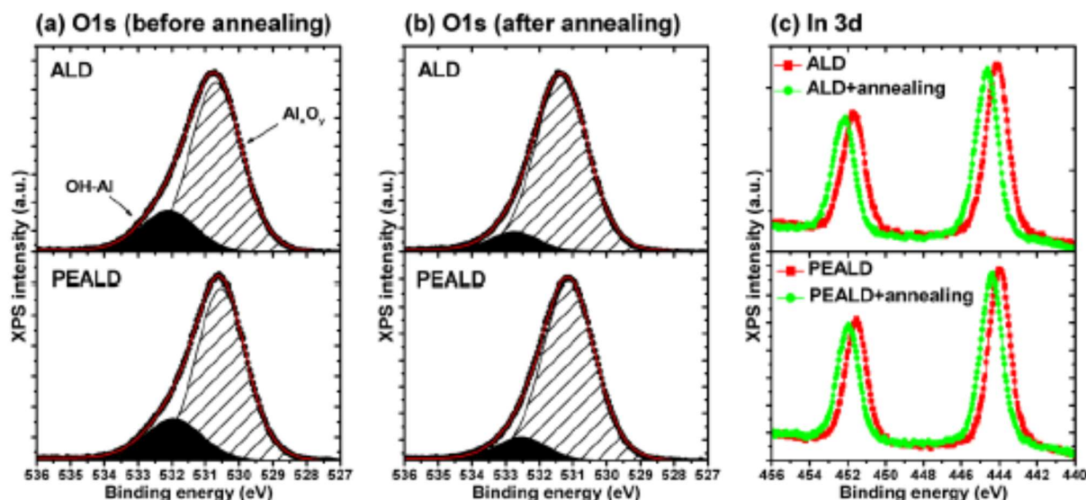
Fig. 10. O1s XPS spectra measured for ALD- \text{Al}_2\text{O}_3/\text{InGaN} and PEALD- \text{Al}_2\text{O}_3/\text{InGaN} samples before (a) and after (b) 400^\circ\text{C} thermal annealing (c) superposition of In3d XPS spectra from the same samples
