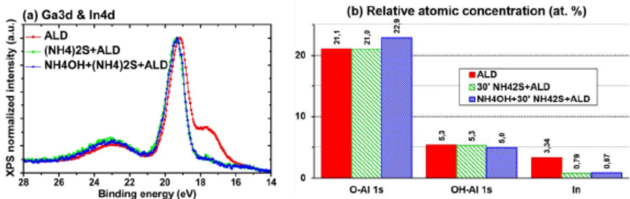
Fig. 9. (a) Superposition of Ga3d & In4d normalized XPS spectra of ALD- \text{Al}_2\text{O}_3 samples without, with a 30' (\text{NH}_4)_2\text{S} or with a \text{NH}_4\text{OH}+30' (\text{NH}_4)_2\text{S} surface treatment (b) Proportion of O1s components and total indium contribution using In4d line
