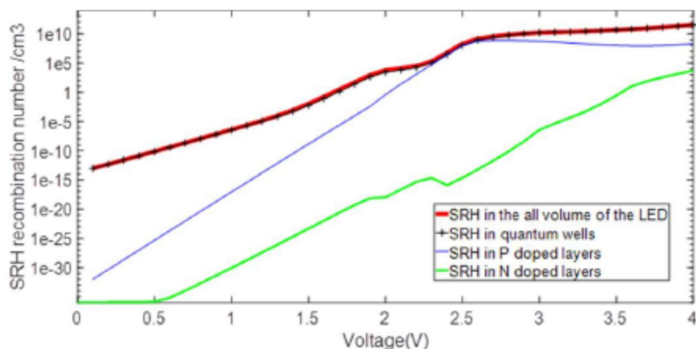
Fig. 1. SRH recombination number/cm 3 in various volumes of a GaN based LED modelled with ATLAS from Silvaco
