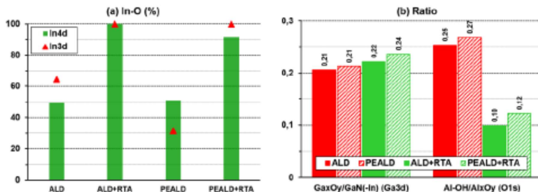
Fig. 11. (a) Estimation of In-O species proportion from indium related peak based on In4d and In3d quantitative analysis for annealed ALD and PEALD samples (b) \text{Ga}_x\text{O}_y/\text{GaN}(-\text{In}) & Al-OH/ \text{Al}_x\text{O}_y ratio for the same samples (respectively from Ga3d and O1s lines)
