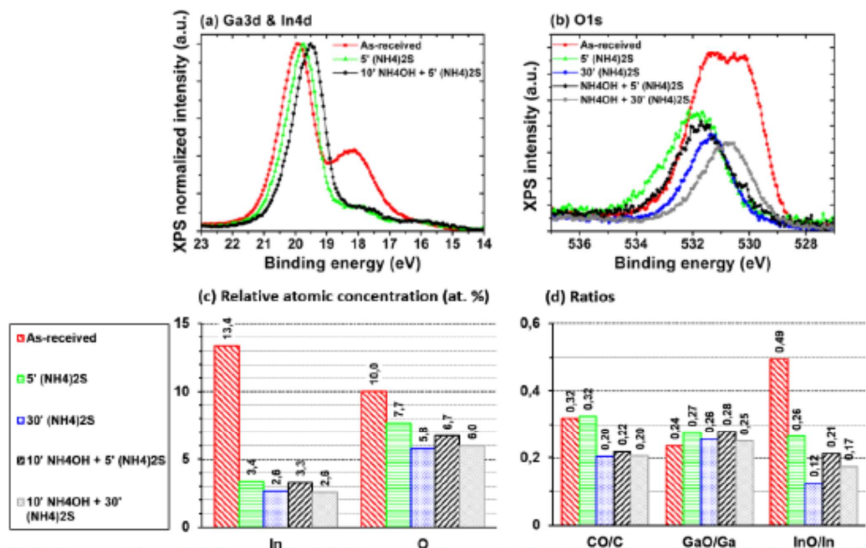
Fig. 4. (a) Superposition of Ga3d normalized XPS spectra of as-received, 5' (NH 4 ) 2 S treated and NH 4 OH + 5' (NH 4 ) 2 S treated samples (b) Superposition of O1s XPS spectra of the same samples and of 30' (NH 4 ) 2 S treated and NH 4 OH + 30' (NH 4 ) 2 S treated samples (c) Indium and oxygen In3d-based stoichiometric analysis (d) Oxidized/unoxidized components ratio
