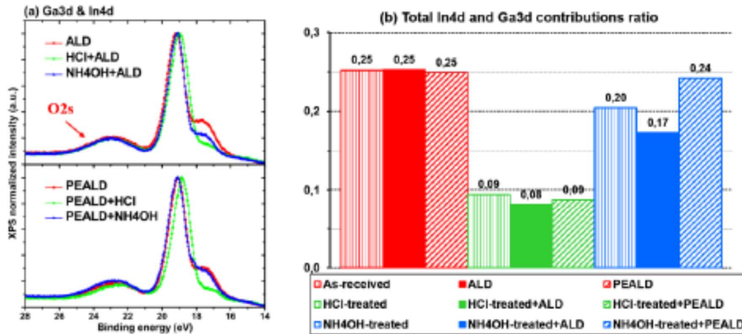
Fig. 8. (a) Superposition of normalized Ga3d-In4d spectra for ALD and PEALD samples without, with HCl or with \text{NH}_4\text{OH} surface treatment (b) In4d/Ga3d ratios for the same samples in comparison with \text{Al}_2\text{O}_3 free surfaces
