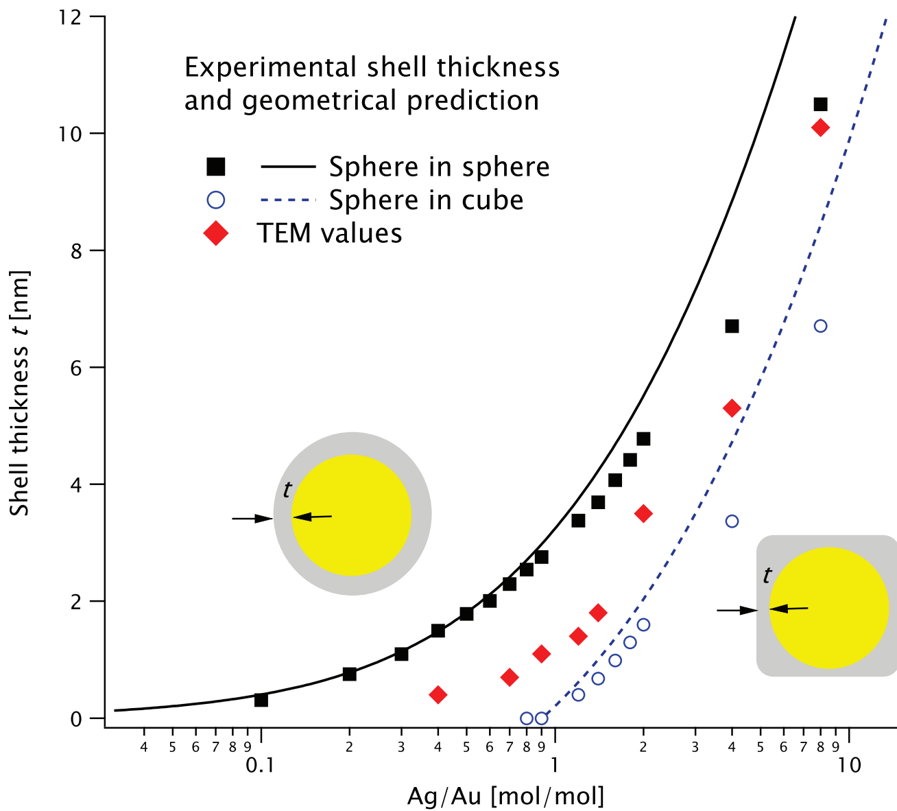
Figure 5 Shell thickness extracted from the fits in Figure 3 for the two models and corresponding geometrical predictions (see the text for more details.) The TEM values are shown as red diamonds.
