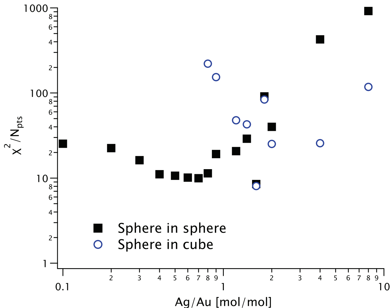
Figure 4 Goodness-of-fit function for the SAXS models in Figure 3, shown as solid squares (for the sphere-in-sphere model) and as open circles (for the sphere-in-cube model) as a function of the Ag/Au ratio K .
