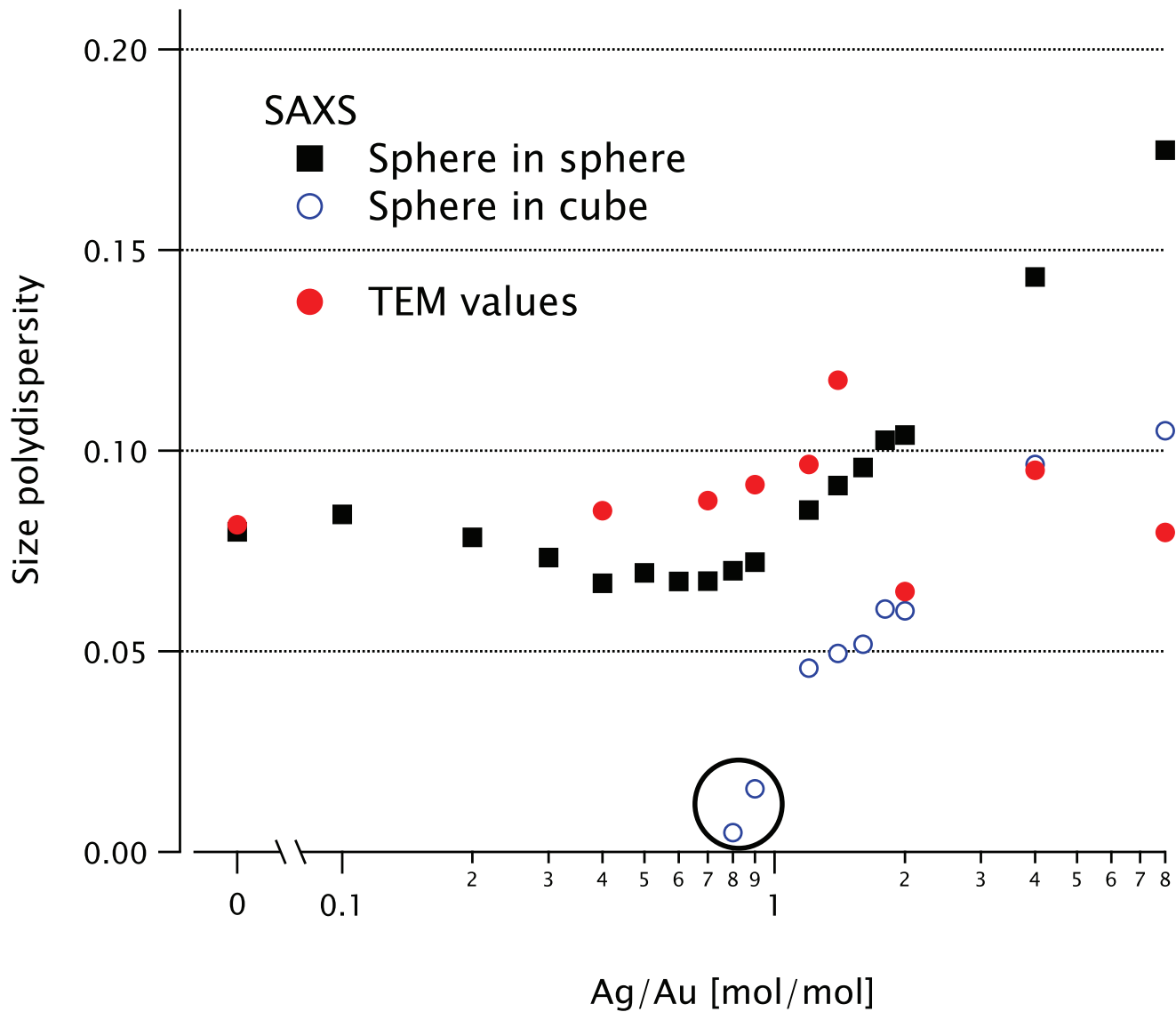
Figure 6 Relative polydispersity extracted from the SAXS fits in Figure 3 for the two models (solid squares for sphere-in-sphere and open dots for sphere-in-cube.) The circled points with abnormally low values (for K = 0.8 and 0.9 ) have very poor fit quality (see Figure 4.) Relative polydispersity extracted from the TEM data (solid dots.)
