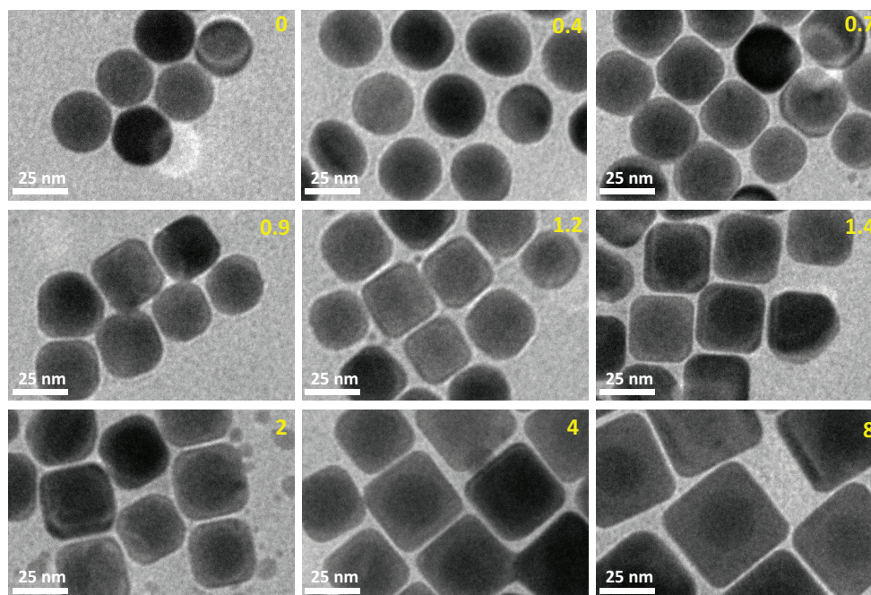
Figure 1 TEM images for different values of the molar ratio K .
