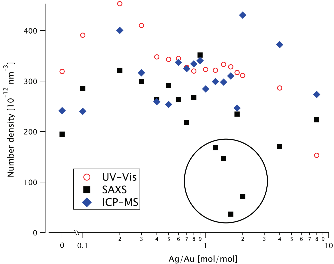
Figure 8 Number particle density n as a function of the Ag/Au ratio K , extracted from fitting the SAXS data in Figure 3 (solid black squares), from the UV-Vis absorbance data (open red dots) and from ICP-MS (blue diamonds). Anomalously low SAXS values are circled.
