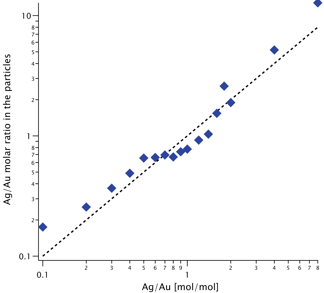
Figure 7 The Ag/Au ratio in the particles, measured by ICP-MS, versus the same ratio in solution, K (diamonds). The dashed line marks the expected values if all the silver is deposited onto the gold cores.
