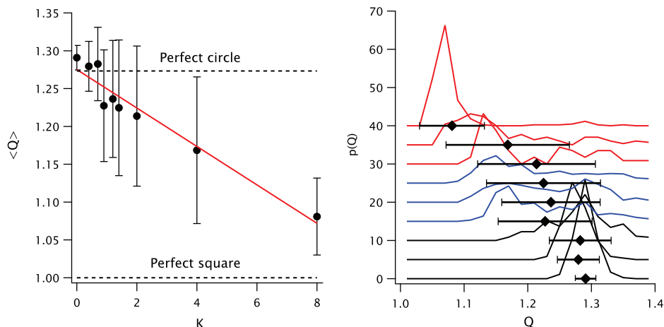
Figure 2 Quadraticity parameter Q . Left: average value \langle Q \rangle as a function of K (mean and standard deviation, solid dots and error bars) with linear fit (solid line). The limiting values for a perfect circle and square are shown as dashed lines. Right: Histograms of Q for each K value (shifted vertically for clarity.) The mean and std. dev. from the left panel are shown under each curve. Colors (black, blue and red) distinguish three types of curves (see text.)
