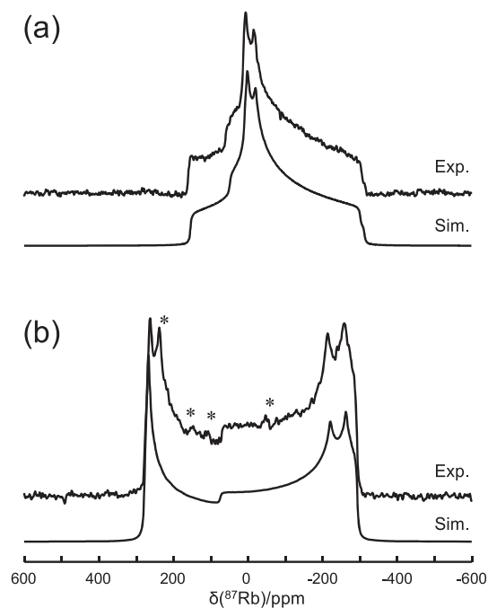
FIGURE 3 Experimental and simulated ^{87}\text{Rb} NMR spectra of static powder samples of (a) \text{Rb}(\text{B15C5})_2\text{Br}\cdot\text{H}_2\text{O} and (b) \text{Rb}(\text{C222})\text{SCN}\cdot\text{H}_2\text{O} at 21.1 T. In each case, 10,240 transients were accumulated with a recycle delay of 1 s. (b) Several sharp features marked by * were likely due to the presence of small microcrystallites
