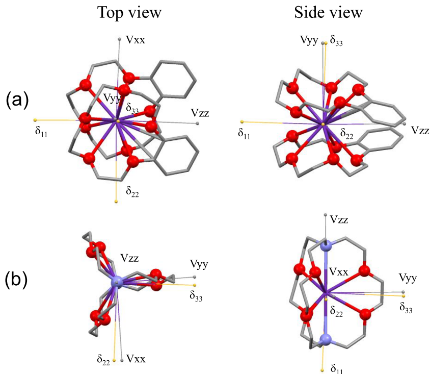
FIGURE 5 Top and side views of the ^{87}\text{Rb} QC and CS tensor orientations in the molecular frame of reference: (a) \text{Rb}(\text{B15C5})_2\text{Br}\cdot\text{H}_2\text{O} and (b) \text{Rb}(\text{C222})\text{SCN}\cdot\text{H}_2\text{O} . Atoms in the first-coordination sphere around the \text{Rb}^+ ion (purple) are highlighted as balls (red, oxygen; blue, nitrogen). All hydrogen atoms are omitted for clarity
