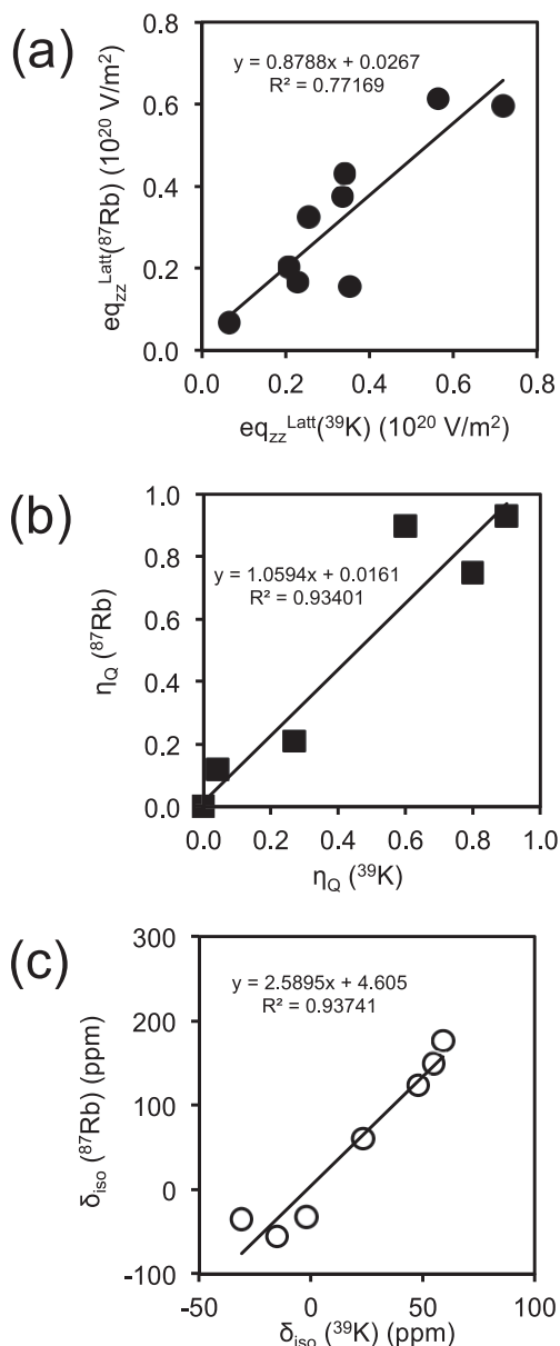
FIGURE 6 Comparison between ^{87}Rb and ^{39}K NMR properties for a series of structurally related Rb + and K + inorganic salts. All experimental values are listed in Tables S1–S3
