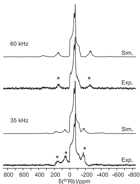
FIGURE 1 Experimental and simulated ^{87}\text{Rb} MAS NMR spectra of \text{Rb}(\text{B15C5})_2\text{Br}\cdot\text{H}_2\text{O} recorded at two sample spinning frequencies at 21.1 T. Spectral features due to spinning sidebands are marked by * in the experimental spectra. Other acquisition parameters are at 35 kHz, 10,000 transients, 0.5-s recycle delay and at 60 kHz, 20,000 transients, 0.5-s recycle delay
