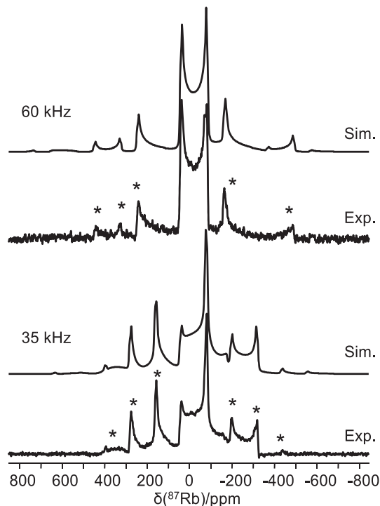
FIGURE 2 Experimental and simulated ^{87}\text{Rb} MAS NMR spectra of \text{Rb}(\text{C222})\text{SCN}\cdot\text{H}_2\text{O} recorded at two sample spinning frequencies at 21.1 T. Spectral features due to spinning sidebands are marked by * in the experimental spectra. Other acquisition parameters are at 35 kHz, 10,000 transients, 0.5-s recycle delay and at 60 kHz, 20,000 transients, 0.5-s recycle delay
