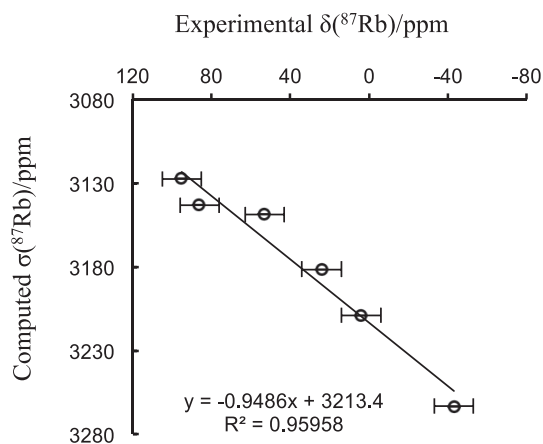
FIGURE 4 Plot of CASTEP computed absolute 87 Rb magnetic shielding ( \sigma ) values against experimental 87 Rb chemical shifts ( \delta ) for Rb(B15C5) 2 Br·H 2 O and Rb(C222)SCN·H 2 O. Note that, because the conversion between magnetic shielding ( \sigma ) and chemical shift ( \delta ) follows \delta = \sigma_{\text{ref}} - \sigma , the y-intercept of the plot yields \sigma_{\text{ref}} = 3213.4 ppm
