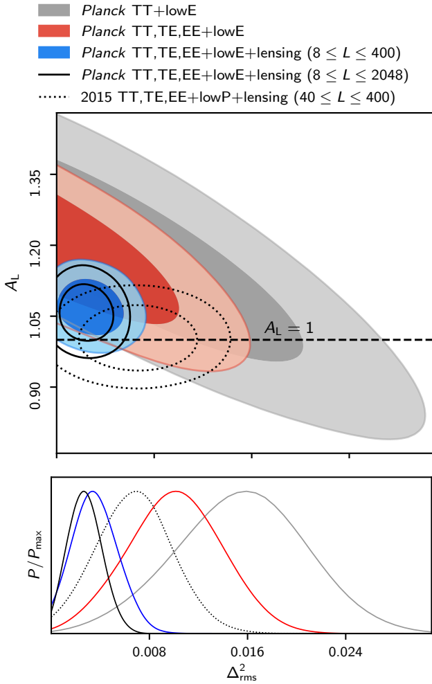
Fig. 47. Degeneracy between A_L and \Delta^2_{rms} in the \Lambda CDM+ A_L +CIP model (top panel) and constraints on \Delta^2_{rms} in the \Lambda CDM+CIP model, where A_L = 1 (bottom panel).
