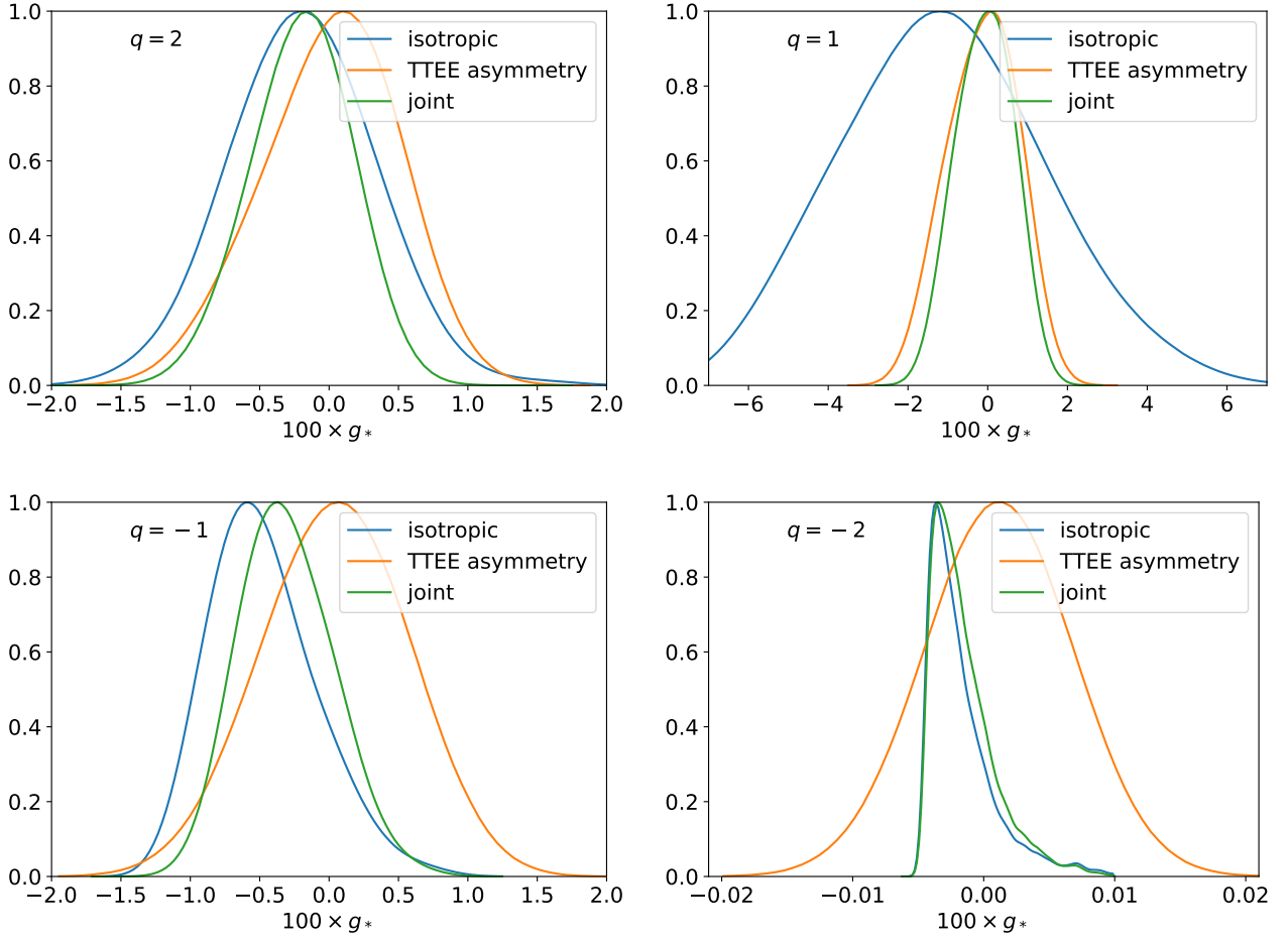
Fig. 50. Marginalized posteriors for quadrupolar modulation parameter g_* , using SMICA data for the TT+EE asymmetry constraints (orange curves) and Planck TT,TE,EE+lowE for the isotropic constraints (blue curves), which probe the modification to the power spectrum via Eq. (114). Top : constraints for q = 2 and 1 (left and right, respectively). Bottom : constraints for q = -1 and -2 (left and right, respectively). Strongly negative g_* is suppressed for q < 0 , due to the unphysical prediction of negative power.
