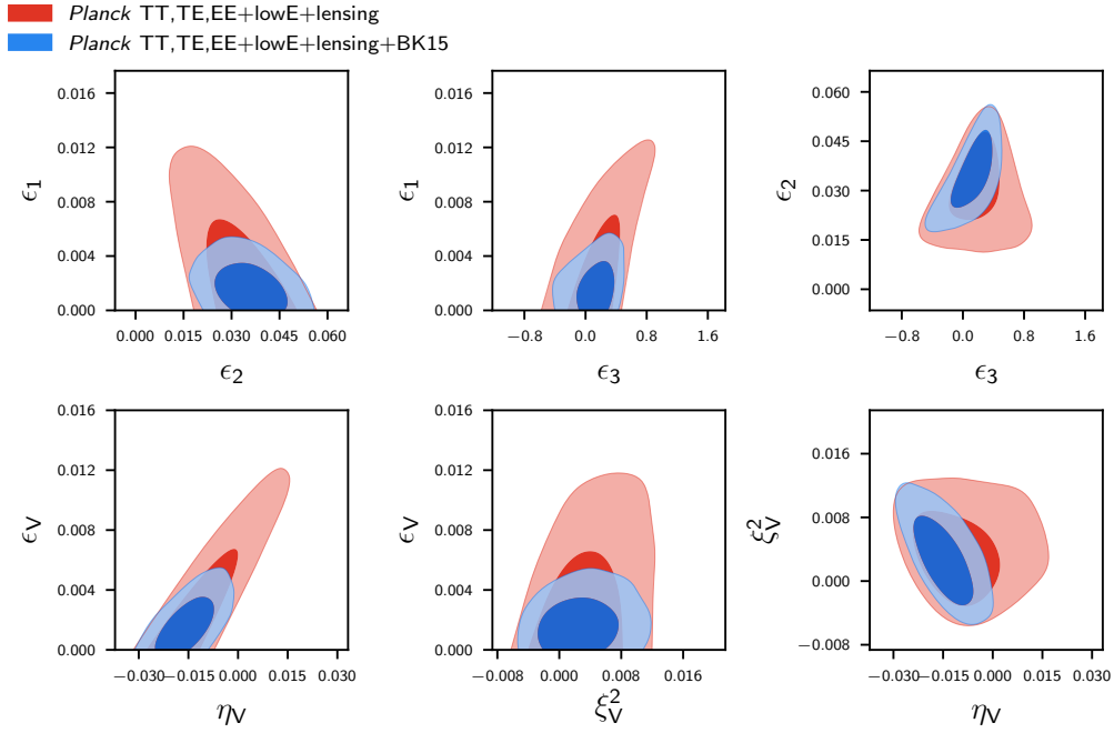
Fig. 7. Marginalized joint two-dimensional 68% and 95% CL regions for combinations of (\epsilon_1, \epsilon_2, \epsilon_3) (upper panels) and (\epsilon_V, \eta_V, \xi_V^2) (lower panels) for Planck TT,TE,EE+lowE+lensing (red contours), compared with Planck TT,TE,EE+lowE+lensing+BK15 (blue contours).
