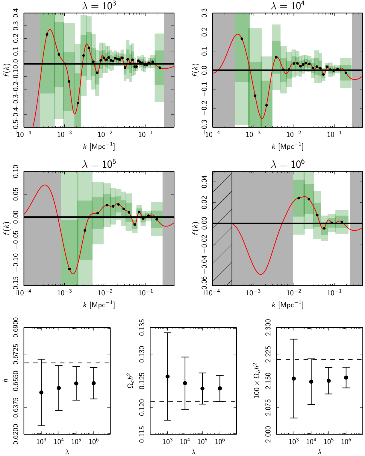
Fig. 18. Planck TT+lowE penalized likelihood primordial power spectrum reconstruction. Top four panels: deviation f(k) for four different roughness penalties. The red curves indicate the best-fit deviation, while the vertical extents of the dark and light green error bars indicate the \pm 1\sigma and \pm 2\sigma errors, respectively. The width of the error bars indicates the minimum reconstructible width (the minimum width for a Gaussian feature such that the mean square deviation of the reconstruction is less than 10%). The grey regions display where the minimum reconstructible width is undefined, meaning that the reconstruction in these regions is untrustworthy. The hatched region in the \lambda = 10^6 plot indicates where the fixing penalty has been applied. Lower three panels: \pm 1\sigma error bars for the three non-primordial-spectrum cosmological parameters included in the reconstruction. The respective best-fit fiducial model values are indicated by the dashed lines.
