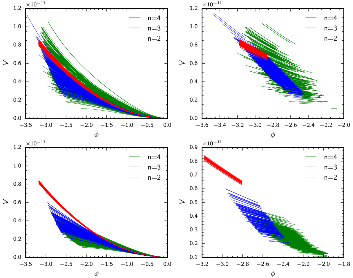
Fig. 16. Representative sample of the inflation potentials allowed at the 95% CL, when the potential is Taylor-expanded at order n = 2, 3 , and 4 and trusted until the end of inflation, and under the assumption of N_* = 55 e -folds of inflation between Hubble-radius crossing for the pivot scale and the end of inflation. In natural units (where \sqrt{8\pi M_{\text{Pl}}} = 1 ). Left panels: full potential from the beginning of the observable window till the end of inflation. Right: zoom on the observable window directly constrained by inflation. Top: Planck TT,TE,EE+lowE. Bottom: Planck TT,TE,EE+lowE+lensing+BK15. Note that there is another branch of solutions that is symmetric under \phi \rightarrow -\phi .
