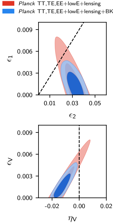
Fig. 6. Marginalized joint two-dimensional 68% and 95% CL regions for (\epsilon_1, \epsilon_2) (top panel) and (\epsilon_V, \eta_V) (bottom panel) for Planck TT,TE,EE+lowE+lensing (red contours), compared with Planck TT,TE,EE+lowE+lensing+BK15 (blue contours). The dashed lines divide between convex and concave potentials.
