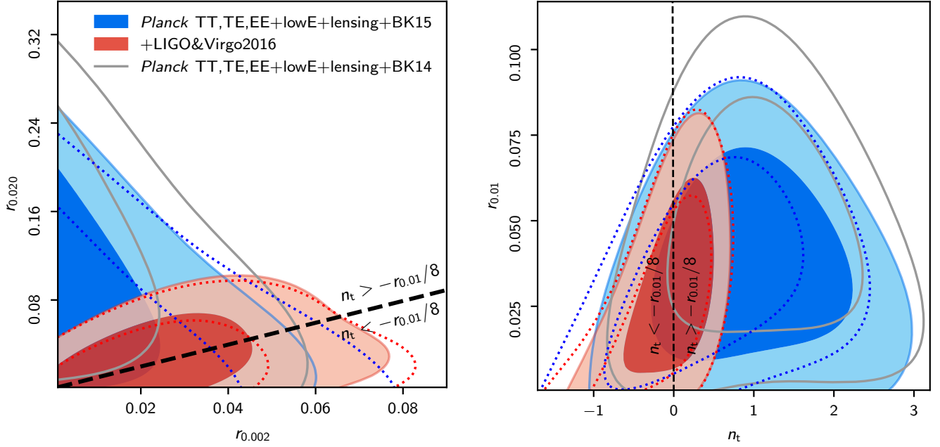
Fig. 5. 68% and 95% CL constraints on tensor perturbations in the \Lambda CDM+ r_{0.002}+r_{0.02} model, i.e., when the inflationary consistency relation is relaxed. Filled contours in the left panel show the results for our independent primary parameters r_{0.002} and r_{0.02} , which have uniform priors, and in the right panel for the derived parameters n_t and r_{0.01} , which have non-uniform priors. The dotted lines assume uniform priors on r_{0.01} and n_t , calculated as in Fig. 4. The scale k = 0.01 \text{ Mpc}^{-1} is near the decorrelation scale of (n_t, r) for the Planck +BK15 data. In both panels the dashed black line indicates the inflationary consistency condition, n_t = -r_{0.01}/8 . (The grey contours follow if we use the older BK14 data instead of the BK15 data.)
