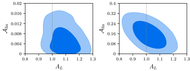
Fig. 29. Marginalized joint 68% and 95% CL regions for the lensing parameter A_L and the modulation amplitude parameter \mathcal{A}_{\text{lin}} using the TT data set. Left : linear oscillation model with \log_{10} \omega_{\text{lin}} = 1.158 and \varphi_{\text{lin}} = \pi . Right : modified linear oscillation model with a Gaussian envelope function (see text) and \log_{10} \omega_{\text{lin}} = 1.158 , \varphi_{\text{lin}} = \pi , \mu_{\text{env}} = 0.2 \text{ Mpc}^{-1} , and \sigma_{\text{env}} = 0.057 \text{ Mpc}^{-1} .
