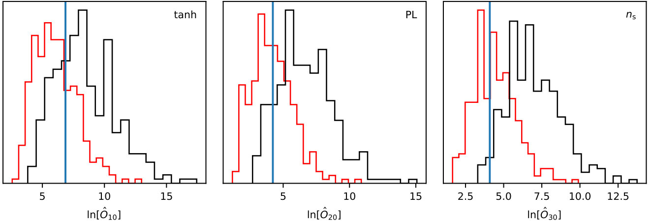
Fig. 49. Histograms of the quantity \hat{O}_{j0} for the tanh, power-law, and n_s gradient modulation models using Planck temperature data combined with 300 statistically isotropic polarization simulations (red outlines) or 300 polarization simulations modulated according to the best-fit parameters from the temperature data (black). The blue lines indicate the values for the actual SMICA polarization data. A large value relative to the isotropic (red) simulations would indicate that the modulation model is preferred over \Lambda CDM.
