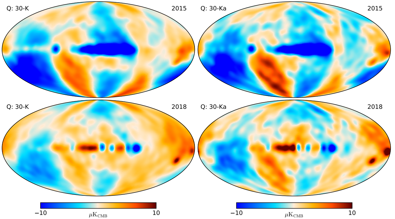
Fig. A.1. Stokes Q difference maps between Planck 30 GHz 2015 ( top ) and 2018 ( bottom ) and WMAP K-band ( left ) and Ka-band ( right ). The WMAP K and Ka band maps are rescaled to match the Planck 30 GHz effective frequency assuming synchrotron emission with a spectral index of -3 . All maps used in this comparison have been smoothed with a 10 deg Gaussian beam.
