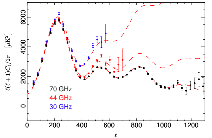
Fig. 20. Binned TT cross-spectra from half-ring maps at 30, 44, and 70 GHz. Foregrounds are accounted for only through the use of the proper frequency-dependent Galactic masks. Red-dashed lines are the Planck best-fit TT spectrum, to which a contribution from unresolved point sources (specific to each frequency) has been added.
