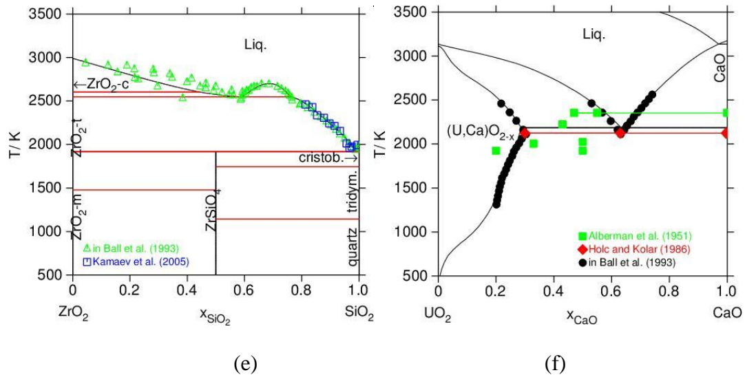
Figure 4: Calculated phase diagrams using the TAF-ID: (a) UO 2 -ZrO 2 section assessed by A. Quaini (b) U-O-Zr at 2273 K section assessed by A. Quaini (c) C-B-Fe liquidus projection from M. Kurata (d) U-B-C at 1500 K assessed by N. Dupin (e) ZrO 2 -SiO 2 assessed by N. Dupin (f) UO 2 -CaO assessed by N. Dupin. A comparison with experimental data is reported when data are available.
