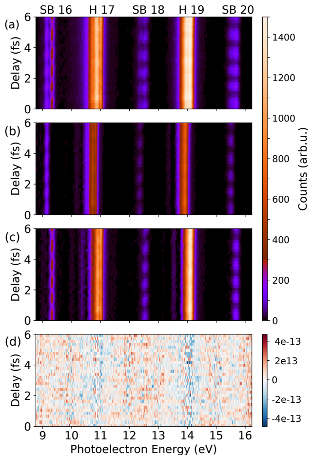
Figure 4: (a) Measured RABBIT spectrogram at \lambda = 791 nm; (b-c) retrieved RABBIT spectrograms for J = 1/2 (b) and for J = 3/2 (c). Differently scaled colormaps are used for sidebands and harmonics for the sake of better visibility. (d) Difference between the measured RABBIT spectrogram and the total retrieved one ( d = a - (b+c) ).
