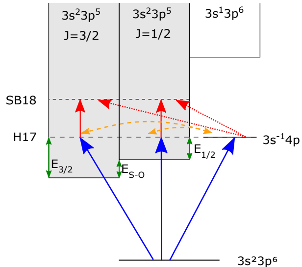
Figure 1: Schematic representation of the energy levels and transitions involved in this work. The blue (red) arrows represent absorption of an XUV (IR) photon. The orange dashed arrows represent the configuration interaction between the quasi-bound state 3s^{-1}4p and the continua. The processes indicated by the red dotted arrows stand for the dipole coupling of the 3s^{-1}4p state with the final continua through absorption of an IR photon. E_{3/2} and E_{1/2} are the kinetic energies of the electrons for different final states of the ion, separated by E_{S-O} .
