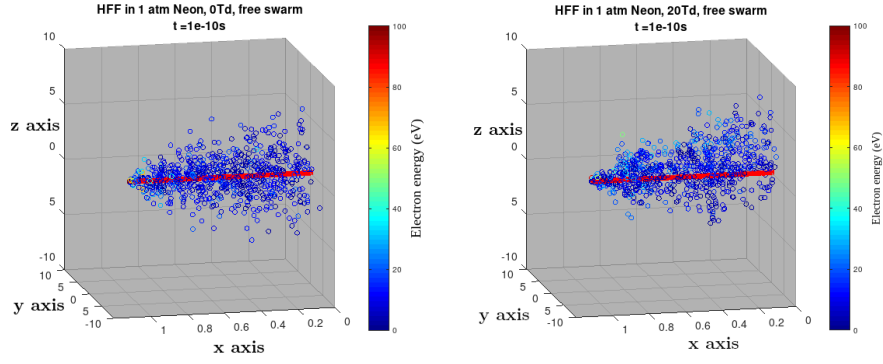
Figure 6: 3-dimension views of the electron swarm energy distribution (colour circles) produced at 100 ps after the emission of a fission fragment (thick red line) without (left) and with (right) an external electric field. X-axis is labelled in mm, y and z-axis in \mu\text{m}
