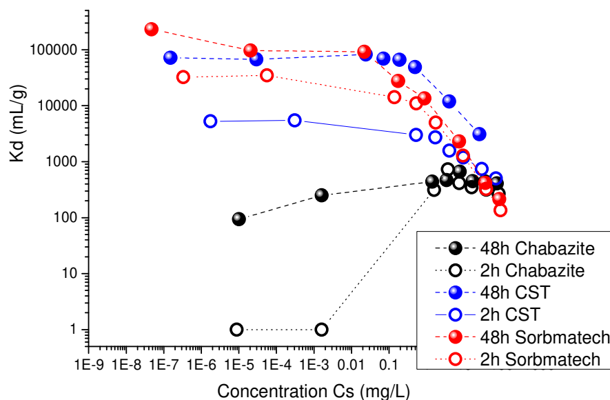
Fig. 3. Cesium distribution coefficients ( K_d ) in the three studied sorbent materials measured after 2 or 48 h in contact with seawater containing different concentrations of either ^{133}\text{Cs} (2-100 \text{mg}\cdot\text{L}^{-1} ) or ^{137}\text{Cs} (trace levels). Sorbmatech, mesoporous silica functionalized with potassium-copper hexacyanoferrate nanoparticles; CST, crystalline silicotitanate.
