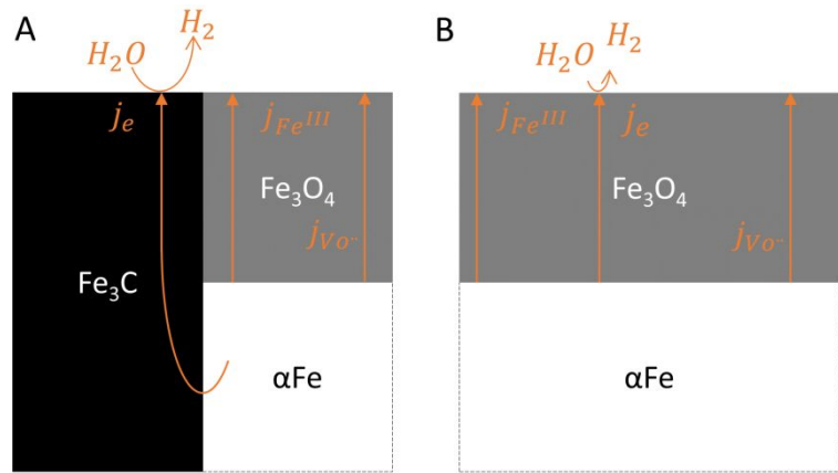
Figure 9- Schematic representation of the diffusion process with (A) and without (B) cementite with j the current of electron e , Fe^{III} and oxygen vacancy vo^{\bullet}
