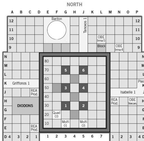
Figure 1. Schematic representation of the core of the OSIRIS reactor in its tank, the six control rods, and the in-core and ex-core experimental positions.
