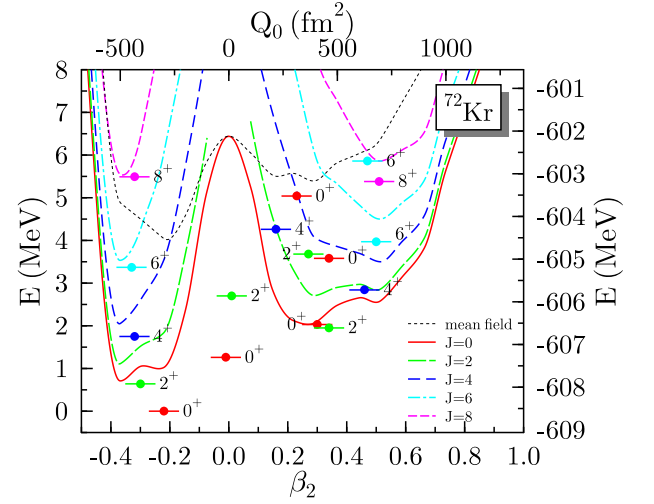
FIG. 15: (color online). Same as Fig. 3 for ^{72}\text{Kr} .
