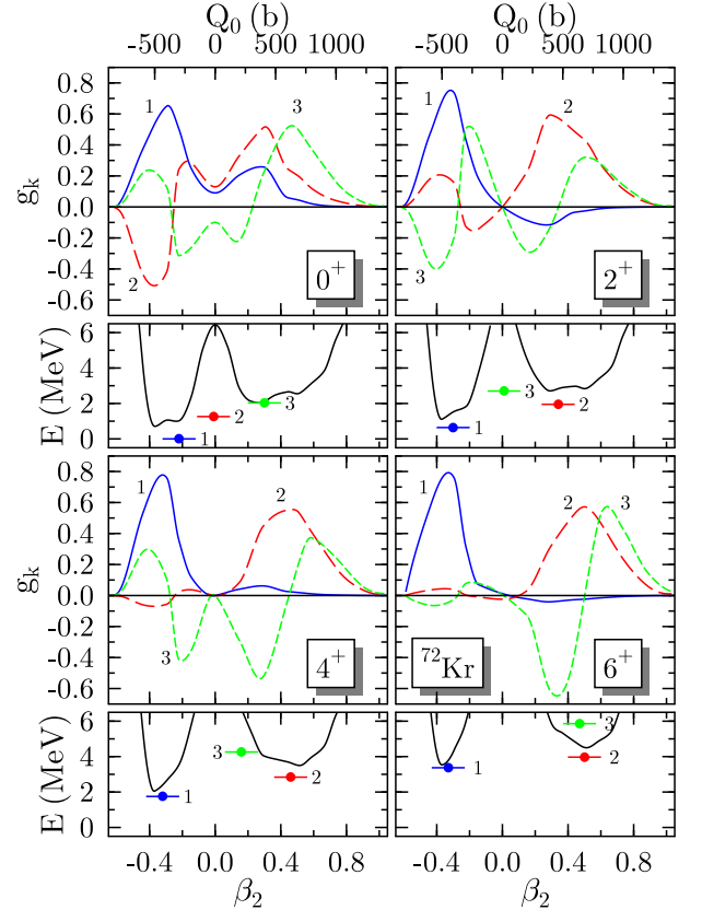
FIG. 16: (color online). The same as Fig. 4 for ^{72}\text{Kr} .
