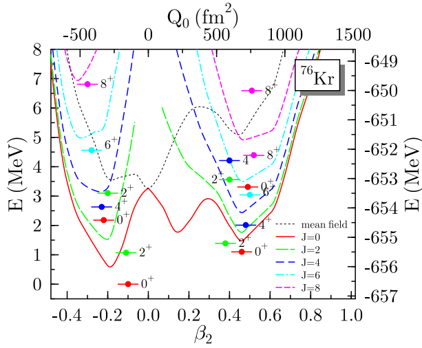
FIG. 7: (color online). The same as Fig. 3 for ^{76}\text{Kr} .
