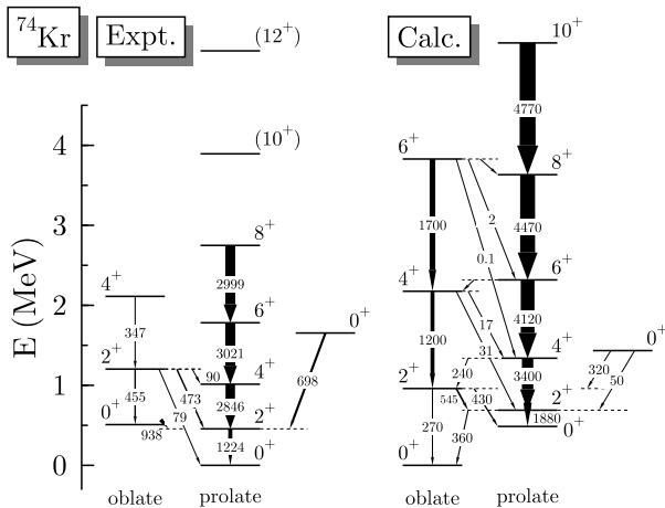
FIG. 5: Spectrum of collective states for ^{74}\text{Kr} as seen in experiment (left) and as obtained from our calculation (right). The arrows with numbers denote the B(E2, J \rightarrow J-2) values for transitions between states with different J and B(E2, J \rightarrow J) for transitions between states with the same J , both given in e^2 \text{ fm}^4 . Experimental values for the B(E2) values are taken from [24, 25]. The labels "oblate" and "prolate" given to the bands correspond to the main components of the collective wave functions.
