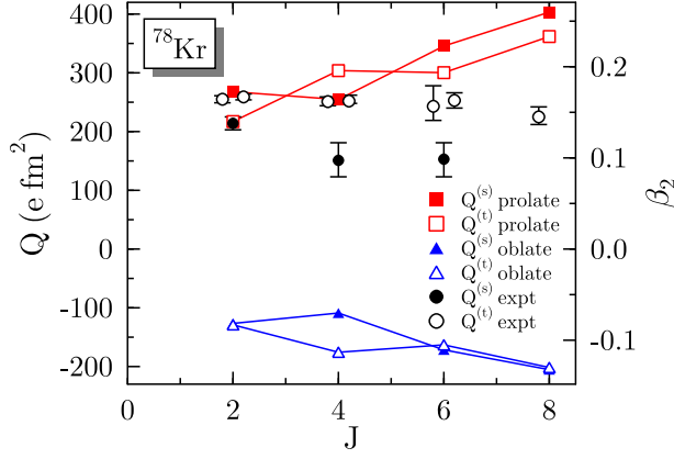
FIG. 14: (color online). Same as Fig. 6, but for ^{78}\text{Kr} . Experimental values are taken from [20, 26].
