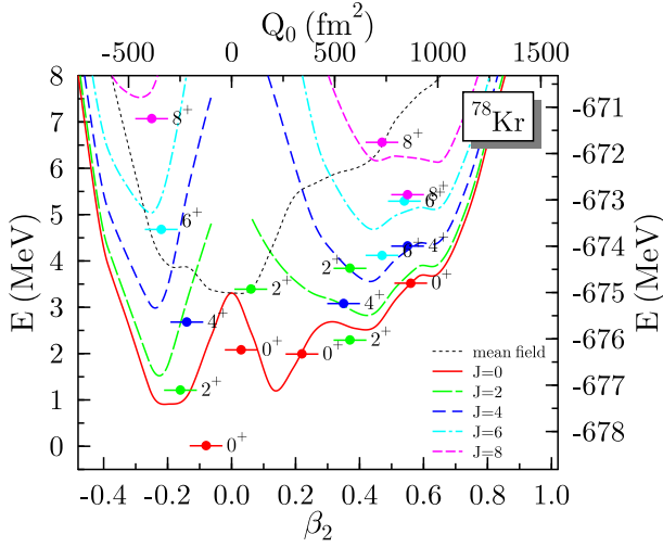
FIG. 11: (color online). Same as Fig. 3, but for ^{78}\text{Kr} .
