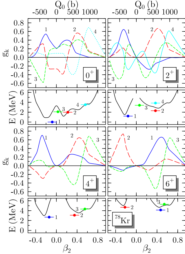
FIG. 12: (color online). Same as Fig. 4, but for ^{78}\text{Kr} .
