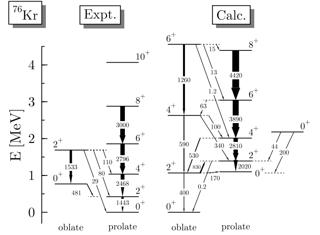
FIG. 9: The same as Fig. 5 for ^{76}\text{Kr} . Experimental data are taken from [25].
