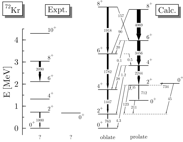
FIG. 17: The same as Fig. 5 for ^{72}\text{Kr} . There is no unambiguous assignment of the experimental yrast states into a prolate or oblate band (see text). Experimental data for the B(E2) values are taken from [18] ( 8^+ \rightarrow 6^+ ) and [22] ( 2_1^+ \rightarrow 0_1^+ ).
