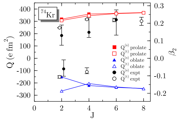
FIG. 6: (color online). Comparison of calculated and experimental Q^{(s)}(J) and Q^{(t)}(J \rightarrow J-2) moments for states in the prolate and oblate bands, assuming that all states are purely axial. Note that -Q^{(t)} is plotted for oblate states for better comparison with Q^{(s)} . Experimental values are taken from [25].
