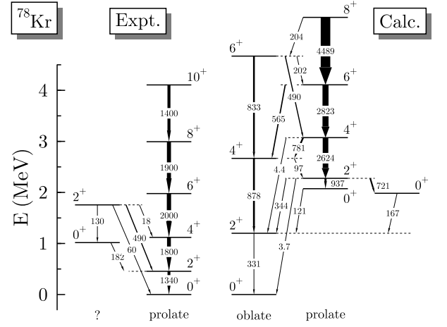
FIG. 13: The same as Fig. 5, but for ^{78}\text{Kr} . Experimental values for the B(E2) values are taken from [26].
