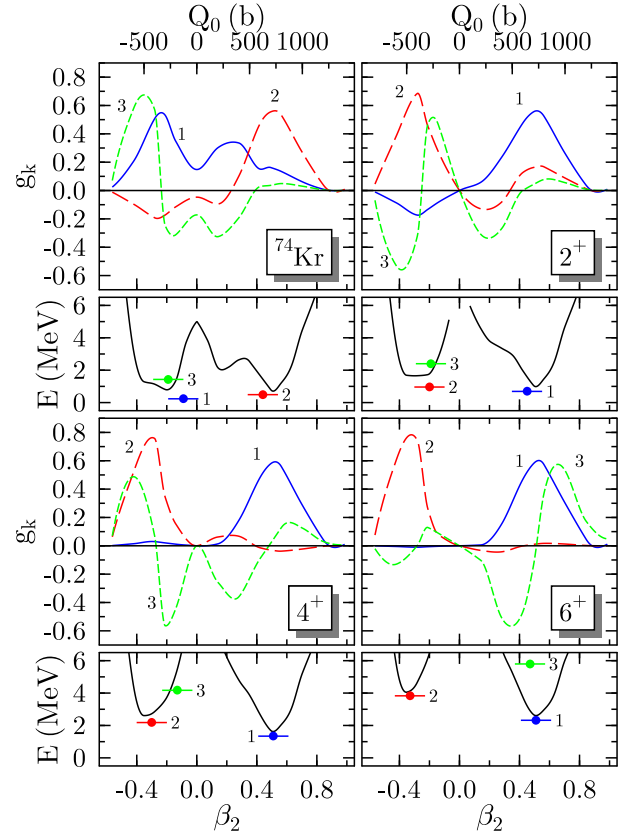
FIG. 4: (color online). Collective wave functions g_k^{(J)} for the lowest states with J = 0, 2, 4 , and 6 for ^{74}\text{Kr} as a function of the intrinsic deformation of the mean-field states they are constructed from. The corresponding energies and average deformations \bar{\beta}_2 are plotted together with the projected energy surface.
