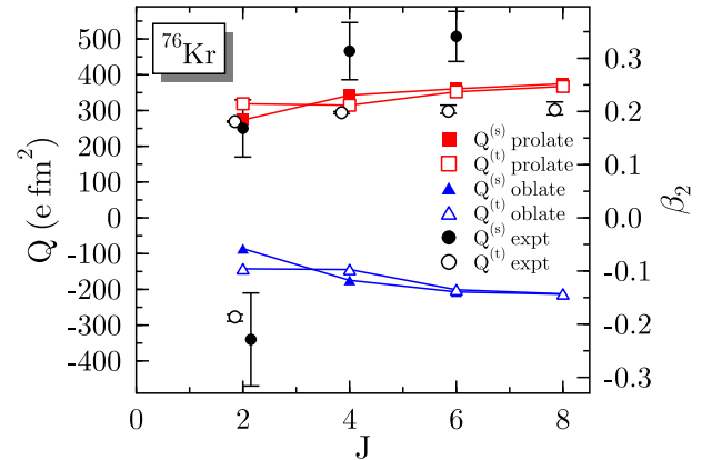
FIG. 10: (color online). Same as Fig. 6, but for ^{76}\text{Kr} . Experimental values are taken from [25].
