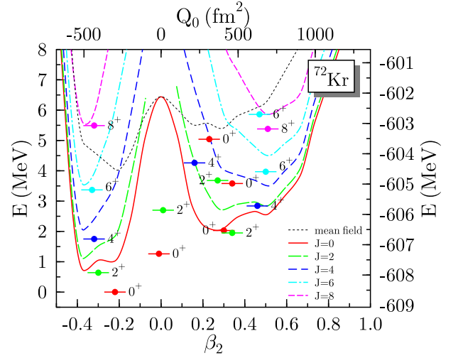
FIG. 15: (color online). Same as Fig. 3 for ^{72}\text{Kr} .
