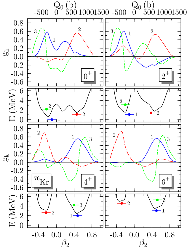
FIG. 8: (color online). The same as Fig. 4 for ^{76}\text{Kr} .
