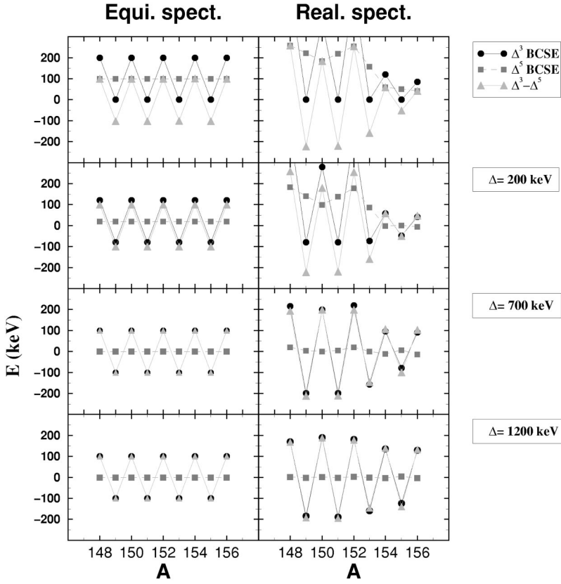
FIG. 10. Energy differences \Delta_{\text{BCSE}}^{(3)} , \Delta_{\text{BCSE}}^{(5)} , and \Delta_{\text{BCS}}^{(3)} - \Delta_{\text{BCS}}^{(5)} . Left and right panels: same as for Fig. 9. The results are displayed between ^{148}\text{Ce} and ^{156}\text{Ce} .
