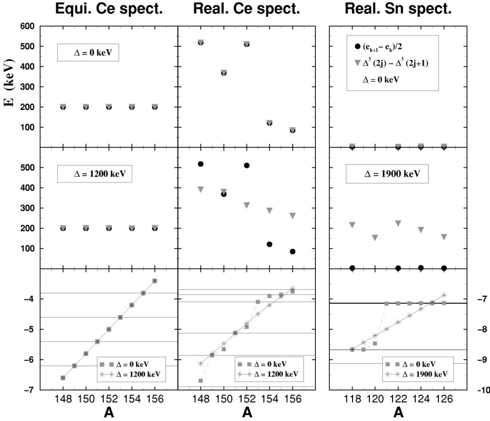
FIG. 13. Upper rows: \Delta^{(3)}(2j) - \Delta^{(3)}(2j+1) compared to the splitting around the Fermi level in the even nucleus (e_{k+1} - e_k)/2 for two extreme values of the gap (top, \Delta = 0 ; middle, \Delta_{realistic} ). The 1.5 MeV splitting for ^{120}\text{Sn} is out of scale. Lower row: chemical potential in MeV as a function of A for the two values of \Delta .
