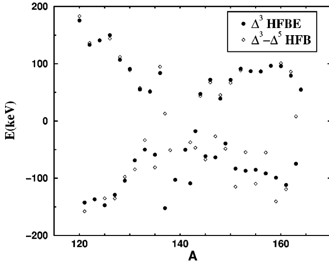
FIG. 8. Comparison between calculated \Delta_{\text{HFBE}}^{(3)}(N) (filled circles) and \Delta_{\text{HFB}}^{(3)}(N) - \Delta_{\text{HFB}}^{(5)}(N) (empty diamonds) along the cerium isotopic line.
