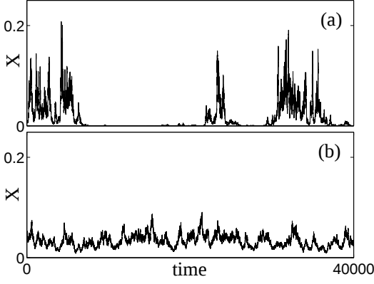
FIG. 1: Temporal traces of the dynamical variable X(t) , solution of (1), with a = 1.25 \times 10^{-3} , \alpha^2 = 0.005 and the noise defined by (6): (a) \eta = \Omega = 0.25 i.e., a/S = 0.3927 ; (b) \eta = \Omega = 2.5 i.e., a/S = 3.9270 .
