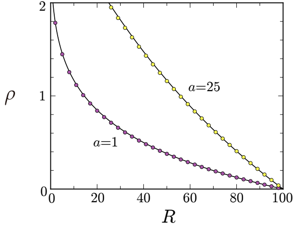
FIG. 4: Stationary density profiles versus R for the GEP with k = 2 in the annulus with external radius L = 100 . Dots are simulation results which were obtained by averaging over 5 \times 10^6 \leq t \leq 10^7 . Solid lines are theoretical predictions given by (37) with \alpha = 1/4 in the case of a = 25 and by (38) when a = 1 .
