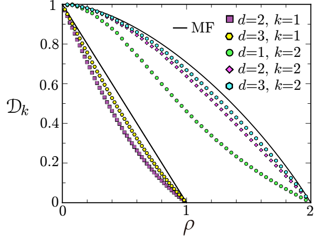
FIG. 7: Coefficient of self-diffusion vs density for the SEP in two and three dimensions, and for the GEP with k = 2 in dimensions d = 1, 2, 3 . Dots represent simulation results. Solid lines are the mean-field predictions: \mathcal{D}_1^{\text{MF}} = 1 - \rho for the SEP, while for the GEP with k = 2 the mean-field prediction \mathcal{D}_2^{\text{MF}} = \Lambda_2(\rho) acquires the explicit form (26).
