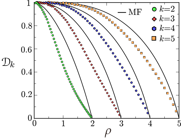
FIG. 6: Coefficient of self-diffusion vs density for the GEP in one dimension; the maximal occupancy varies between k = 2 and k = 5 . Dots represent simulation results for the GEP in one dimension. Solid lines are the mean-field predictions, Eq. (52).
