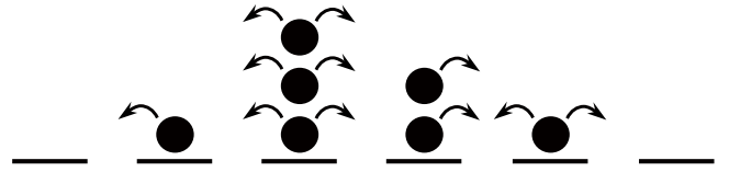
FIG. 1: GEP with k = 3 in one dimension. Hopping into a site occupied by three particles is forbidden; other hopping events occur with the same (unit) rate. Thus the total hopping rate from every site is equal to the number of particles at the site times the number of neighboring sites which are not fully occupied.
