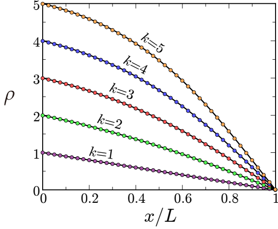
FIG. 3: Stationary density profiles versus x/L for the GEP with k = 1, 2, 3, 4, 5 on a segment with L = 10^3 . The solid lines are theoretical predictions in the case of extremal boundary densities, \rho_0 = k and \rho_1 = 0 . For the SEP ( k = 1 ), the density profile is linear; for k = 2 , the density profile is given by (33), and generally it is extracted from Eq. (35). Simulation results (shown by \bullet ) were obtained by averaging over the time window 5 \times 10^6 \leq t \leq 10^7 .
