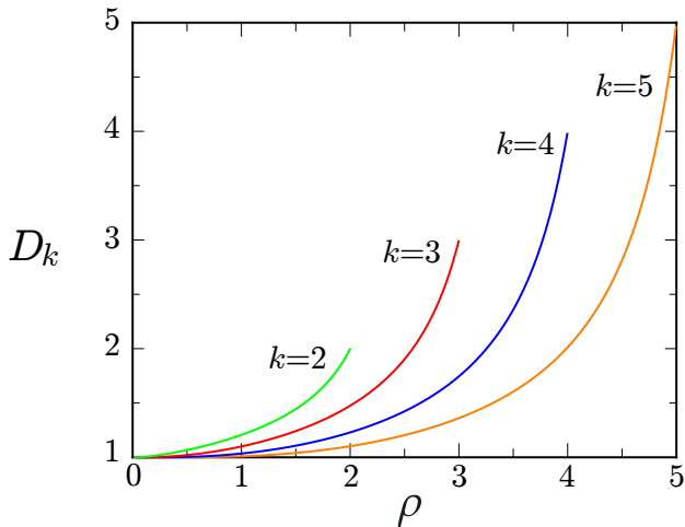
FIG. 2: Diffusion coefficient (7) as a function of density for the GEP with k = 2, 3, 4, 5 .
