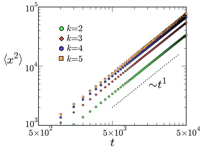
FIG. 5: Mean-square displacement of the tagged particle vs time for the GEP in one dimension. The maximal occupancy varies between k = 2 and k = 5 . Simulations were performed on the ring of length 10^3 .
