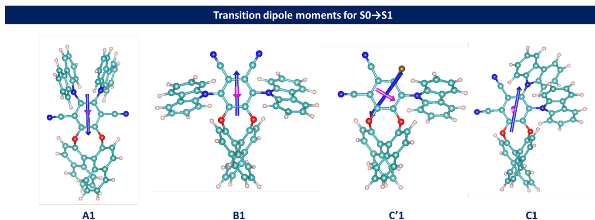
Figure 5: Schematic representation of electric (blue) and magnetic (magenta) transition dipole moments of the S_0 \rightarrow S_1 transition.
