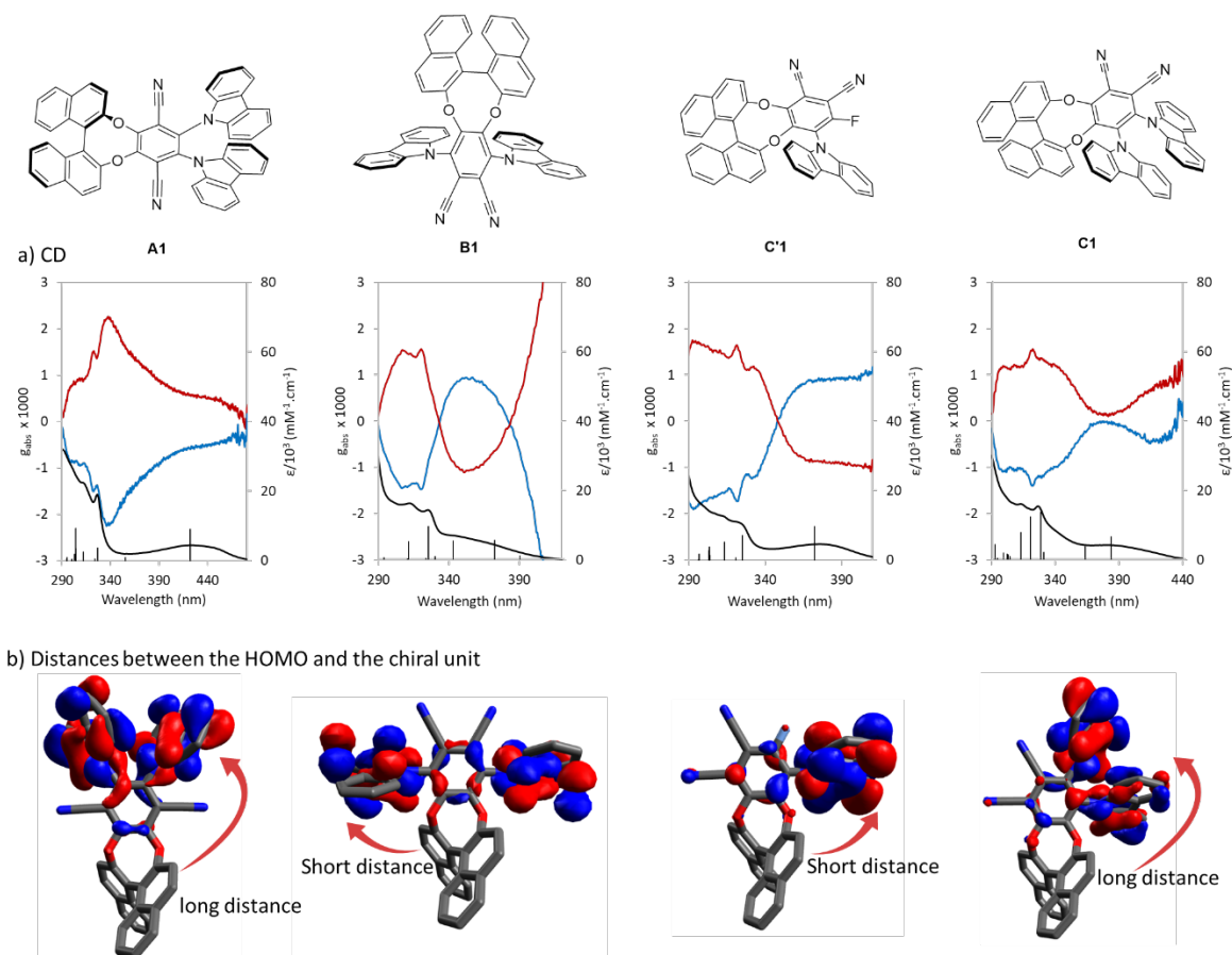
Figure 4: Influence of isomerism on chiroptical properties: a) UV (in black) and g_{abs} (color) spectra measured in toluene at 1 mM, oscillator strengths are plotted to visualize transitions but are not scaled. For g_{abs} = f(\text{nm}) blue traces correspond to molecules with ( R )- configuration and red traces correspond to molecules with ( S )-configuration; b) HOMO of the 4 different isomers.
