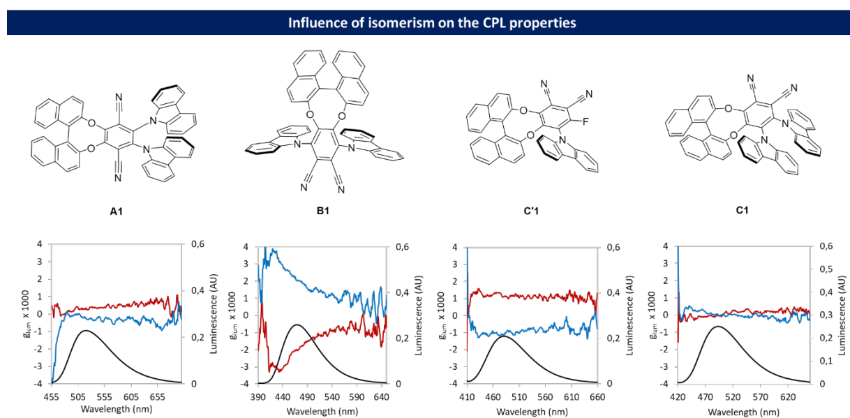
Figure 6: Influence of isomerism on the chiroptical properties at the excited state. g_{\text{lum}} = f(\text{nm}) in toluene solution, blue traces correspond to molecules with ( R )- configuration and red traces correspond to molecules with ( S )-configuration; black traces correspond to fluorescence spectra. For A1 , g_{\text{lum}} remains almost constant along the emission band centered at 520 nm with a value of 0.4 \times 10^{-3} . [17] Surprisingly, for isomer B1 , the g_{\text{lum}} value tends to decrease with the emission wavelength. Relatively high values of g_{\text{lum}} were measured with a maximum of 3.0 \times 10^{-3} at the beginning of the emission band and a value of 2.0 \times 10^{-3} at 472 nm ( \lambda_{\text{em}} \text{ max} ). For isomer C'1 the values of g_{\text{lum}} remain roughly constant along the emission band centered at 493 nm with a value of 1.0 \times 10^{-3} . Isomers C1 shows very low values of g_{\text{lum}} nearing zero at \lambda_{\text{em}} \text{ max} with an unusual bisignate pattern. The influence of the carbazole substituents on chiroptical properties
