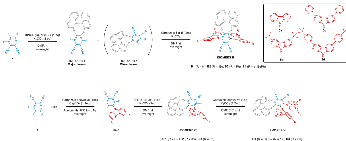
Scheme 1: Synthesis of isomers B , C' and C
