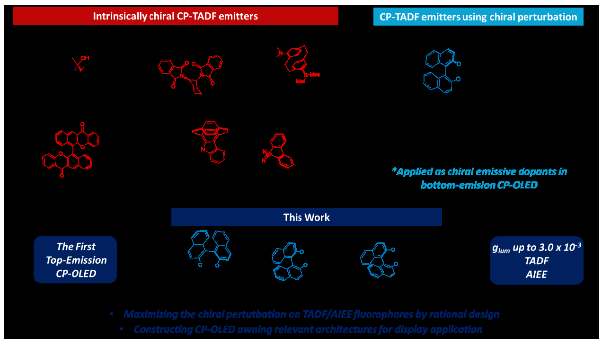
Figure 1: Molecular designs reported so far to construct CP-TADF molecules ( g_{lum} values reported in toluene solution) and new molecular designs explored in this work.
