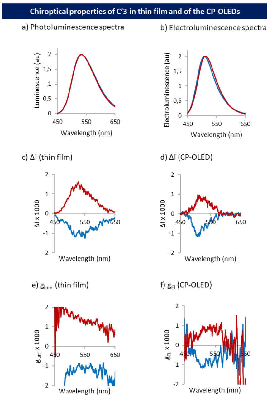
Figure 10: a) photoluminescence response of single layers of pure C'3 ; b) electroluminescence response of the top-emission CP-OLEDs; c) \Delta I = f(\text{nm}) curves related to single layers of pure C'3 ; d) \Delta I = f(\text{nm}) curves related to the electroluminescence generated by the CP-OLEDs; e) g_{lum} = f(\text{nm}) curves obtained for single layers of pure C'3 ; f) g_{EL} = f(\text{nm}) curves related to the electroluminescence generated by the top-emission CP-OLEDs; red traces correspond to molecules with ( S )- configuration and blue traces correspond to molecules with ( R )-configuration.
