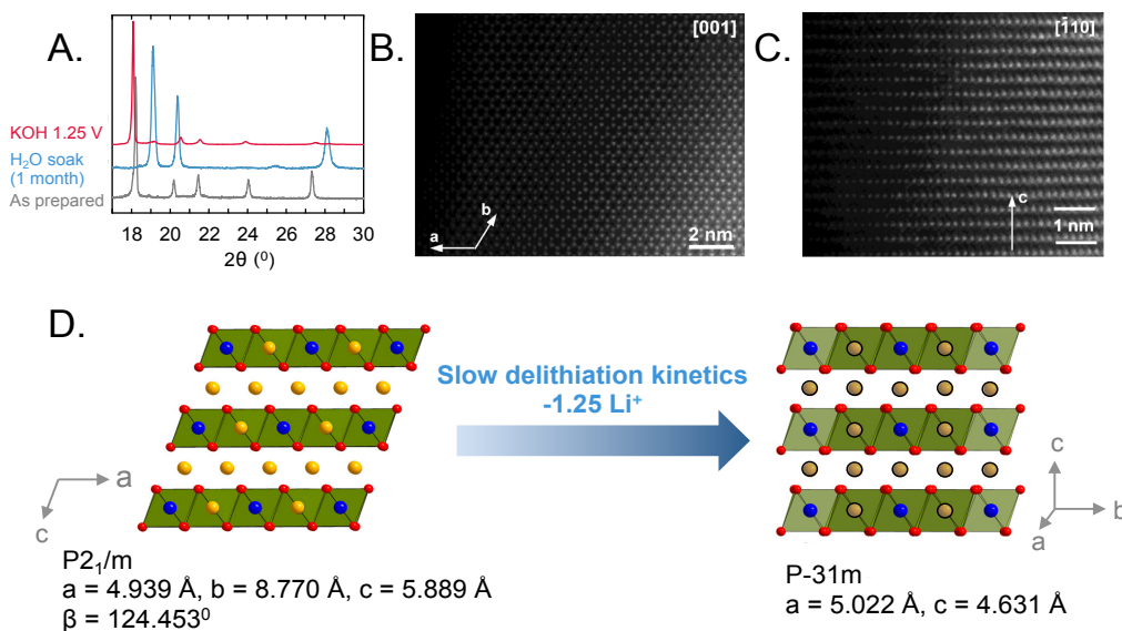
Figure 6: (A) XRD pattern of a pure delithiated phase synthesized by two different methods – the O3-“Li 1.4 RuO 3 ” phase in red synthesized by electrochemical delithiation at 1.25 V RHE in 0.1 M KOH and the O1-“Li 0.75 H 1.25 RuO 3 ” phase in blue synthesized by soaking pristine Li 2 RuO 3 in water for 1 month. (B) [001] HAADF-STEM image of perfect “honeycomb” ordering. (C) [-110] HAADF-STEM image showing a sequence of the hexagonal close-packed layers typical of the O1 structure. (D) Schematic indicating that slow delithiation kinetics upon exposure of as-prepared Li 2 RuO 3 to water results in the transformation of the O3 structure to an O1 hexagonal close packed structure. Blue, red and yellow spheres represent Ru, O and Li respectively. Exchangeable cations are shown in grey on the right, where these sites can be filled with Li or H.
