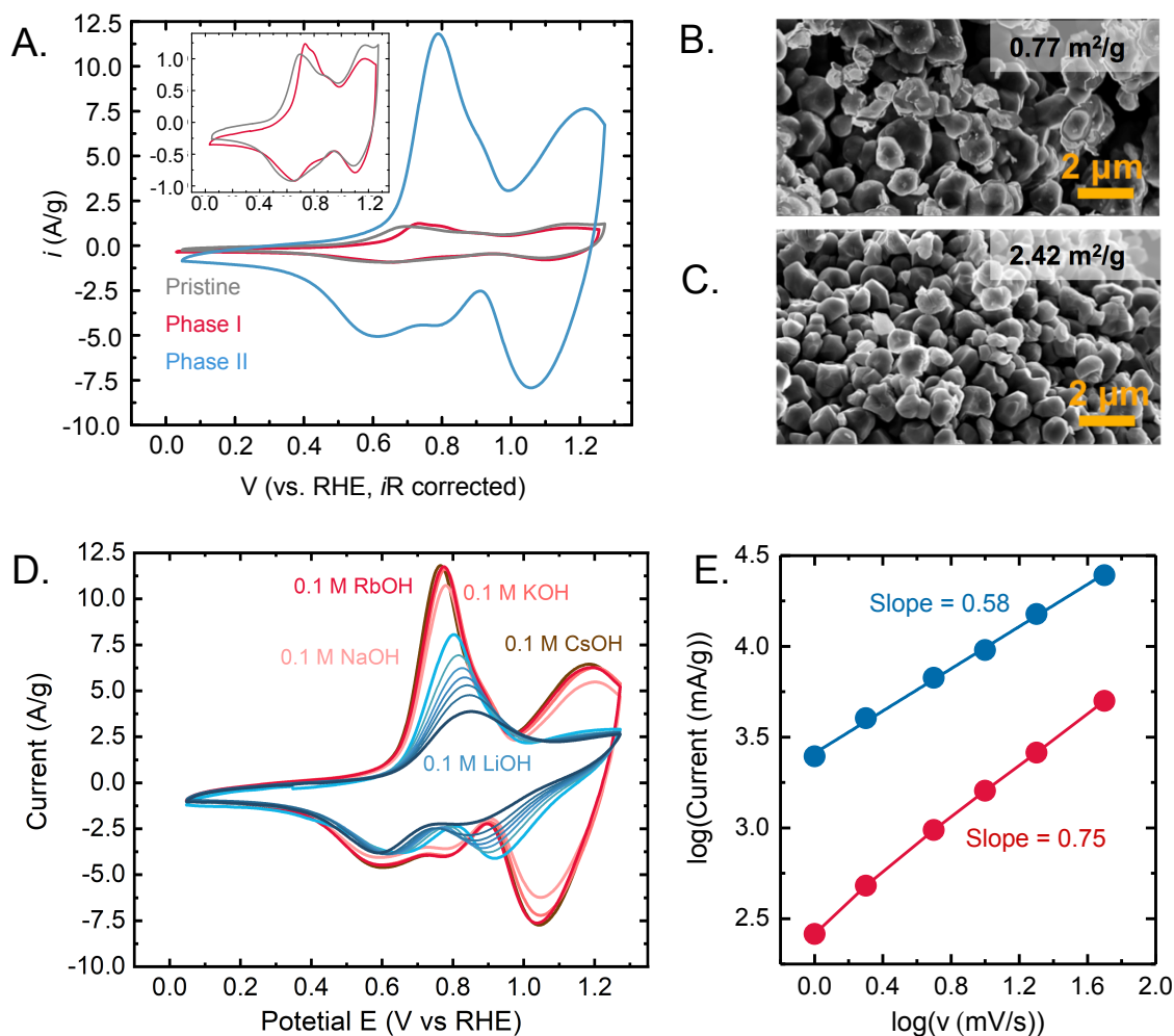
Figure 5: (A) Cyclic voltammograms at 10 mV/s of as-prepared \text{Li}_2\text{RuO}_3 (in grey), “ \text{Li}_{1.4}\text{RuO}_3 ” (in red) and “ \text{Li}_{0.75}\text{H}_{1.25}\text{RuO}_3 ” (in blue) synthesized by holding at 1.25 V_{\text{RHE}} in Ar-saturated 0.1 M KOH for 48 hours and soaking in water for ~30 days respectively. Oxide particles were deposited on a glassy carbon disk and the nominal oxide loading was 0.255 \text{ mg}_{\text{oxide}}/\text{cm}_{\text{disk}}^2 . Helium ion microscopy images of the particles for the (B) as prepared and (C) “O1- \text{Li}_{0.75}\text{H}_{1.25}\text{RuO}_3 ” in water shows that exposure to water results in breakdown of particles causing a three-fold increase in surface area. (D) Cyclic voltammograms for the “O1- \text{Li}_{0.75}\text{H}_{1.25}\text{RuO}_3 ” sample in Ar-saturated 0.1 M LiOH, NaOH, KOH, RbOH and CsOH at 10 mV/s. The presence of Li ions in solution results in a decrease in the redox peak currents with cycling (increasing scans are indicated by darker shades of blue). However, there is no change in the bulk structure of the sample soaked in a Li containing solution for a period of ~1 month. This suggests that the influence of Li results in a chemical/structural modification of the surface/interface of the electrode, causing loss of the redox currents (E) Variation of the log of the peak current as a function of the log of the scan rate for the anodic redox peak at \sim 0.7 V_{\text{RHE}} for “ \text{Li}_{1.4}\text{RuO}_3 ” (in red) and “ \text{Li}_{0.75}\text{H}_{1.25}\text{RuO}_3 ” (in blue). A value of 0.5 for the slope suggests
