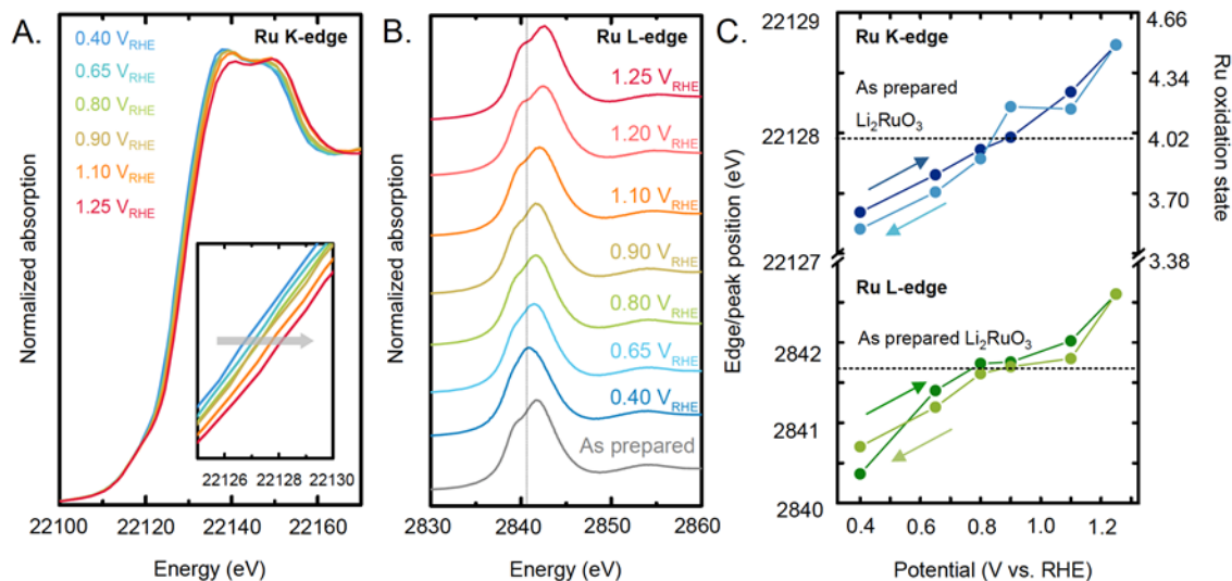
Figure 4: In situ X-ray absorption spectroscopy data in 0.1 M KOH of (A) Ru K-edge (22.117 keV) in fluorescence mode with an acquisition angle of approximately 45^\circ . Time of acquisition of one spectrum is \sim 30 min (B) Ru L 3 -edge (2.8379 keV) in fluorescence mode with an acquisition angle of approximately 45^\circ . Time of acquisition of one spectrum is \sim 50 min. Measurements were first collected at open circuit potential and then the potential was increased from 0.4 V RHE to 1.25 V RHE and decreased back to 0.4 V RHE . The working electrode is a glassy carbon where a mix of Li 2 RuO 3 and carbon with volume ratio of 1:19 was deposited, to form a thin layer of \sim 10 \mu\text{m} thick. The reference electrode is Ag/AgCl. (C) The shift in the edge position (for the K-edge) and the peak position (for the L-edge) suggests oxidation of bulk Ru with increasing potential. The Ru oxidation state corresponding to the Ru K-edge shift has been extracted from previous work. [47]
