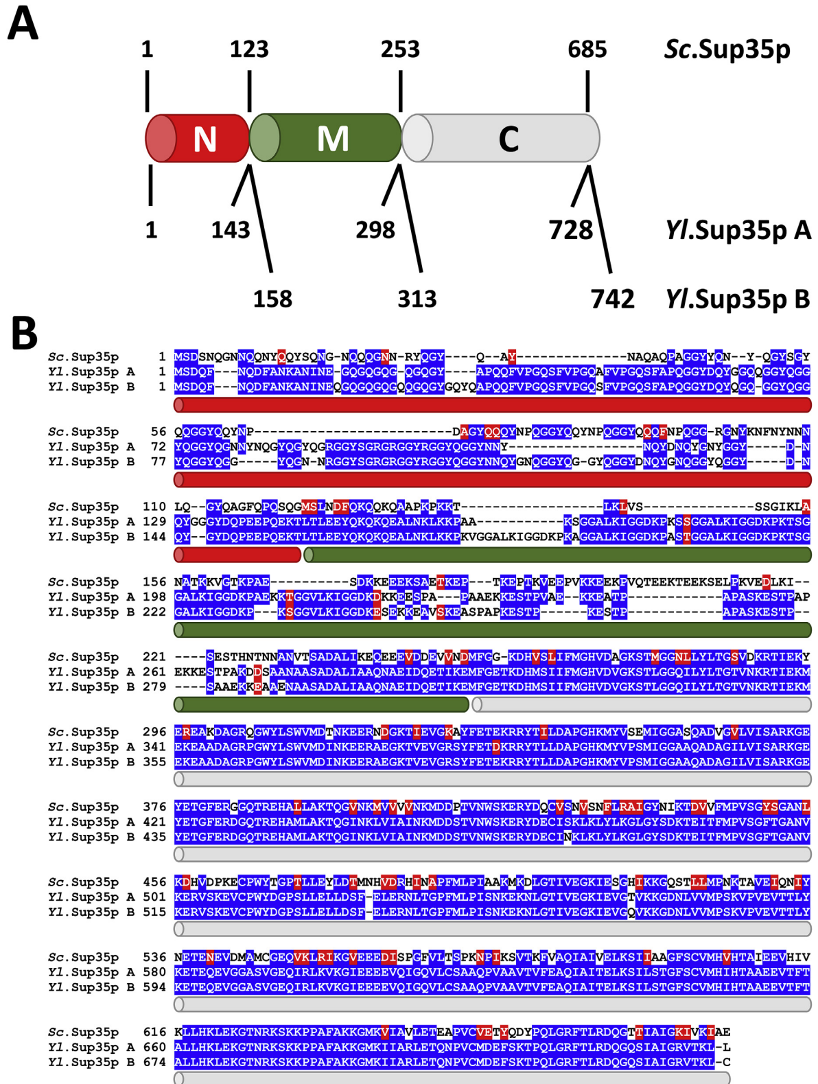
Fig. 1. Alignment of Sc.Sup35p, Yl.Sup35p A and Yl.Sup35p B proteins. The S. cerevisiae Sc.Sup35p coding sequence (Uniprot P05453) was obtained from the 74-D694 strain. The Yl.Sup35p A coding sequence was obtained from Y. lipolytica strains 136,463 and PO1d (Uniprot Q6CFC9). The Yl.Sup35p B coding sequence was obtained from Y. lipolytica strain SS397A (accession number AB039752). (A) Primary structure and domain organization of Sc.Sup35p, Yl.Sup35p A and Yl.Sup35p B proteins (see text for details). (B) Sequence alignment of Sc.Sup35p, Yl.Sup35p A and Yl.Sup35p B proteins (the alignment was made using T-COFFEE and BOXSHADE).
