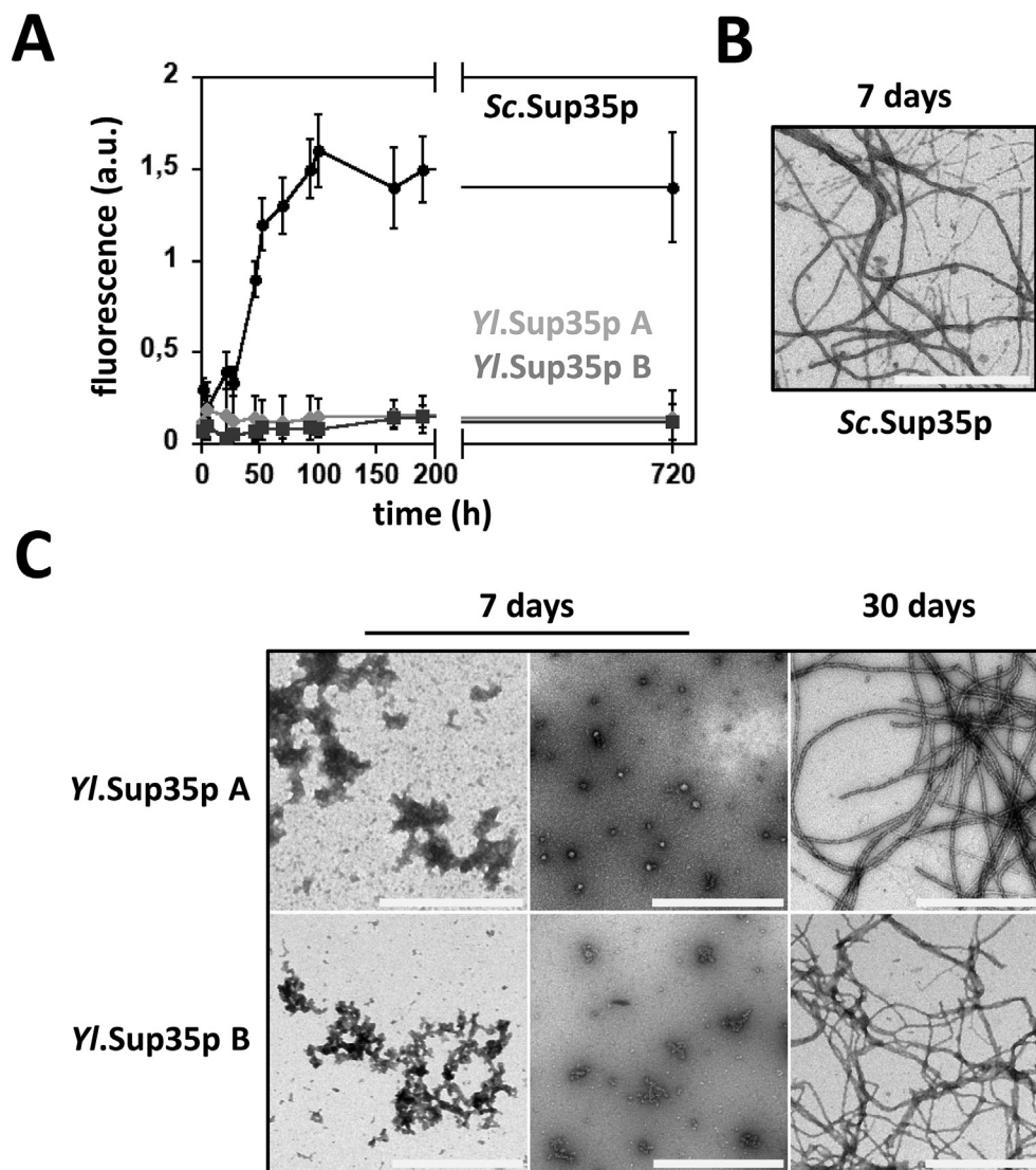
Fig. 2. Assembly of full-length Y. lipolytica and S. cerevisiae Sup35p proteins. (A) Full-length Y. lipolytica and S. cerevisiae Sup35 proteins were allowed to assemble at a final concentration of 10 \mu\text{M} and at 6 ^{\circ}\text{C} under very low agitation (<100 rpm). Aliquots were removed at regular time intervals and assayed using the Thioflavin T binding assay described in the Materials and Methods section. (B, C) Assembly reactions were imaged at the indicated time points using negative-stained electron microscopy (scale bars, 1 \mu\text{m} ).
