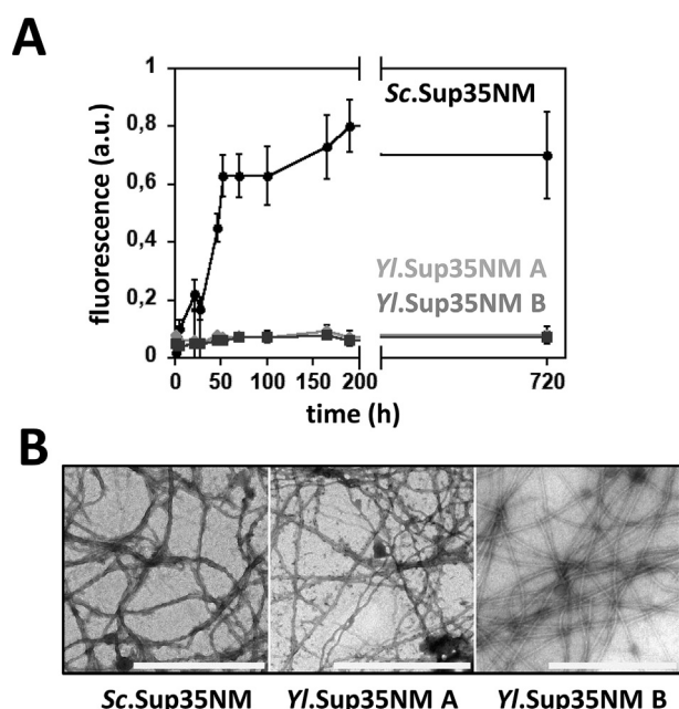
Fig. 4. Assembly of Y. lipolytica and S. cerevisiae Sup35NM proteins. (A) The indicated purified proteins were allowed to assemble at a final concentration of 10 \mu M at 6 °C under very low agitation (<100 rpm). Aliquots were removed at regular time intervals and assayed using the Thioflavin T binding assay described in the Materials and Methods section. (B) Sc.Sup35NM (7 days), Yl.Sup35NM A and Yl.Sup35NM B (30 days) fibril preparations were imaged using negative-stained electron microscopy (scale bars, 1 \mu m).
