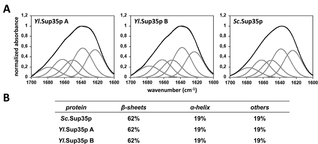
Fig. 3. FT-IR spectra of fibrillar Y. lipolytica and S. cerevisiae Sup35 proteins. (A) The recorded FT-IR spectra (black lines) and curve fit data (grey lines) are shown for fibrillar Y. lipolytica and S. cerevisiae Sup35 proteins. The spectra were fitted using a Gaussian species model centered at 1624, 1640, 1652, 1664 and 1678 cm -1 . (B) Secondary structure content of S. cerevisiae and Y. lipolytica Sup35p fibrils derived from the deconvolution of the FTIR data presented in (A).
