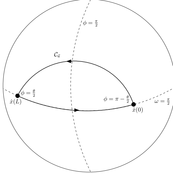
Figure 14. Phase factor for the saddle-point solution. Schematic representation of the path \vec{u}(\nu) , see Eqs. (B.15) and (B.19). The phase \Phi(\mathcal{C}_{\vec{u}}) is given by the area enclosed by the path.
