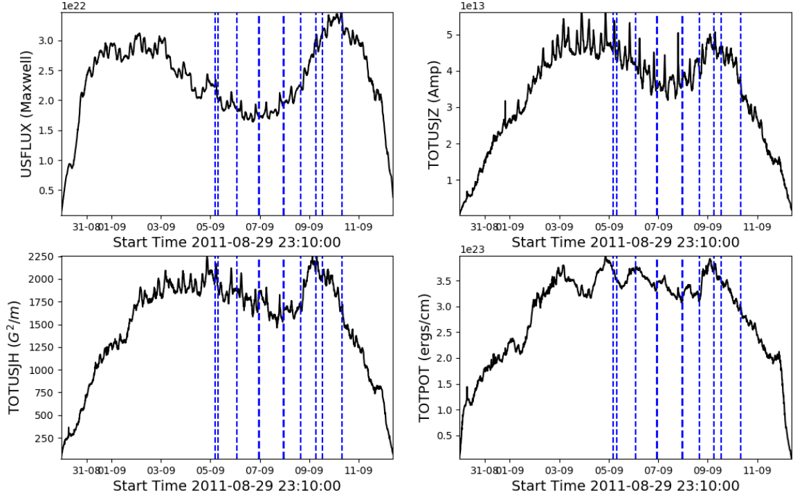
Fig. 2. Time evolution of the total unsigned magnetic flux (USFLUX), the total unsigned vertical current (TOTUSJZ), the total unsigned current helicity (TOTUSJH), and the total photospheric magnetic free-energy density (TOTPOT) for active region NOAA 11283 (SHARP 833). The thick dashed vertical blue line corresponds to an X-class solar flare, and the thin dashed vertical blue line corresponds to an M-class solar flare.
