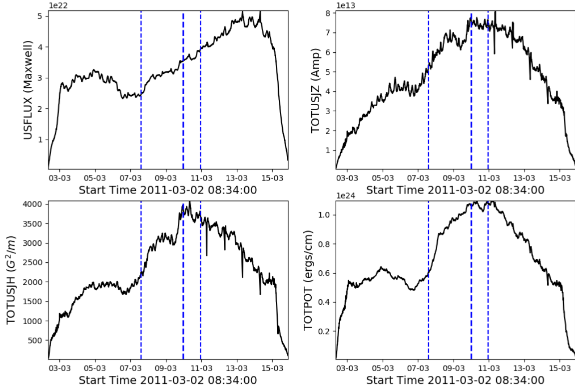
Fig. 1. Time evolution of the total unsigned magnetic flux (USFLUX), the total unsigned vertical current (TOTUSJZ), the total unsigned current helicity (TOTUSJH), and the total photospheric magnetic free-energy density (TOTPOT) for active region NOAA 11166 (SHARP 401). The thick dashed vertical blue line corresponds to an X-class solar flare, and the thin dashed vertical blue line corresponds to an M-class solar flare.
