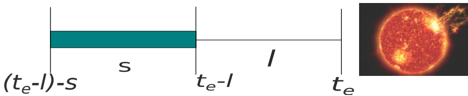
Fig. 4. Data selection criteria for eruptive active regions in terms of flare-generating time ( t_e ), loopback time ( l ), and span time ( s ). We use the time evolution of the active region parameters during span time ( s ) to train the machine-learning algorithm. The loopback time is also the forecasting window.
