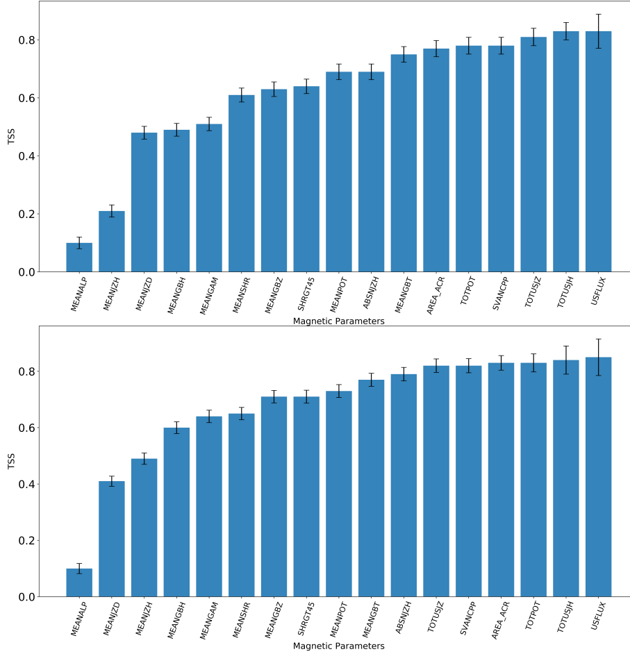
Fig. 5. Top bar plot: distribution of TSS values after running the logistic regression (baseline) classifier on the summarized time series of individual active region parameters. Bottom bar plot: same, but for the support vector machine algorithm. This plots clearly show that the top few parameters, specifically, the total unsigned magnetic flux and the total unsigned magnetic helicity, have the best distinguishing capability.
