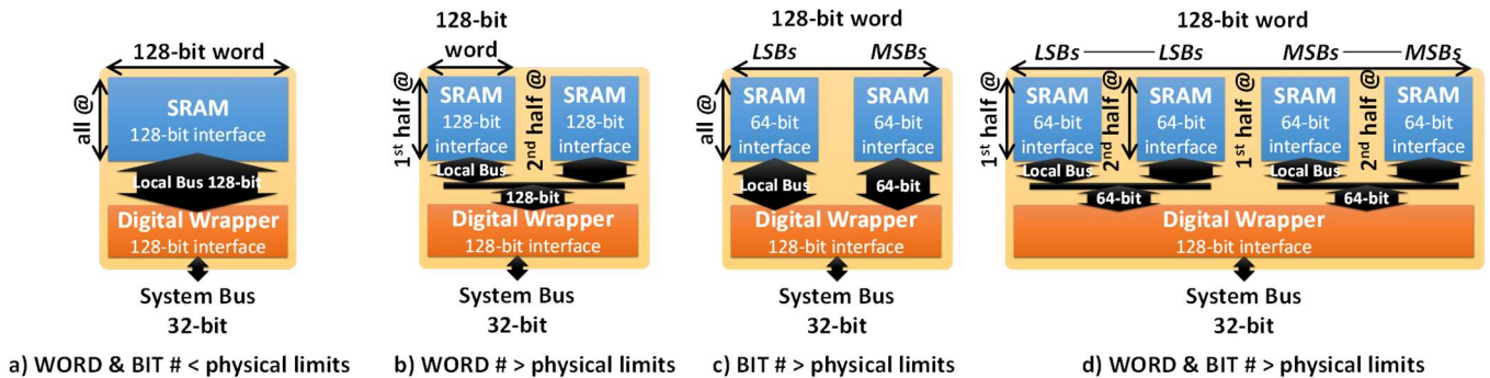
Figure 3 128-bit SRAM cut partitioning constrained by the physical limitations: a) word & bit number < physical limits, b) word number > physical limits, c) bit number > physical limits and d) word & bit number > physical limits.
