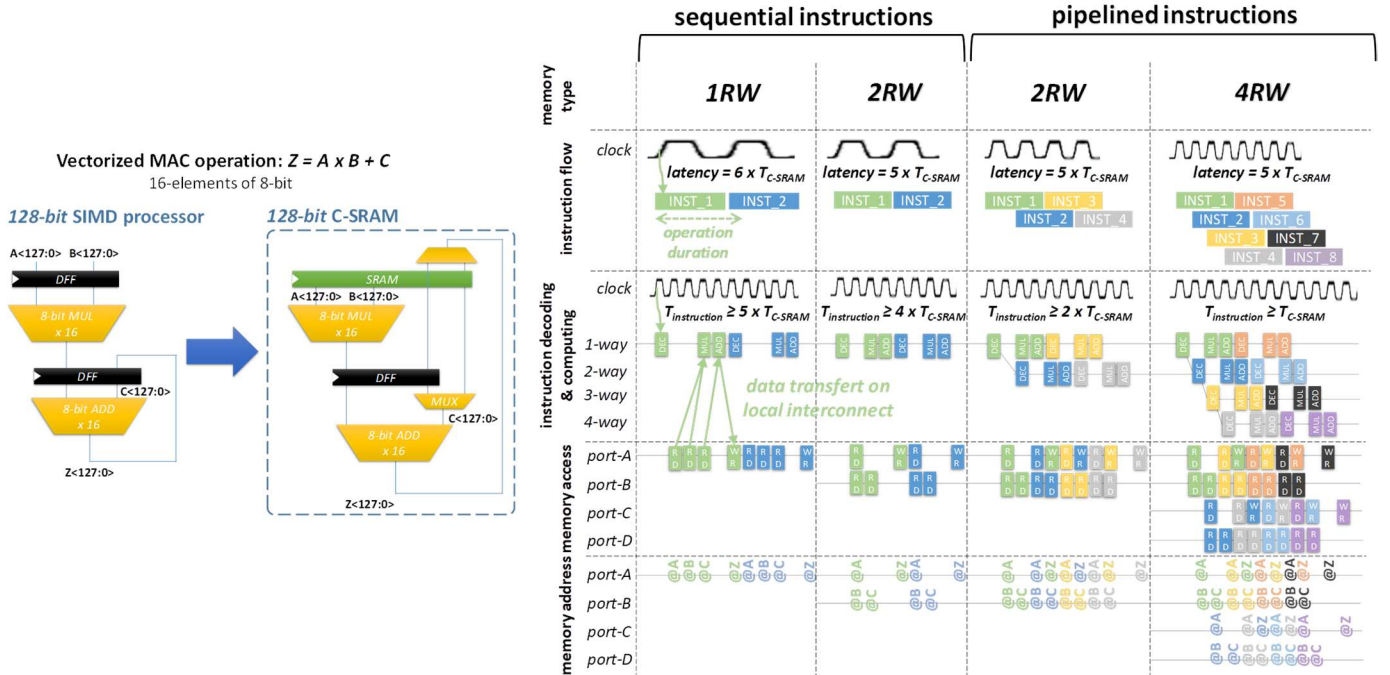
Figure 7 Chronogram of the multiply-accumulate operation ( Z = A * B + C ) performed with various C-SRAM configurations. These configurations depend on the selected SRAM type (1RW, 1R1W ...), the frequency ratio between C-SRAM and instruction flow and the way the instructions are performed in the digital wrapper (pipeline enabled or not).
