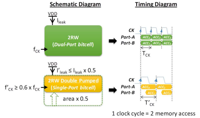
Figure 5 Basic concept of the double pumping technique enabling the port number duplication, while keeping a clock frequency ratio \geq 0.6 w.r.t. the reference solution.
