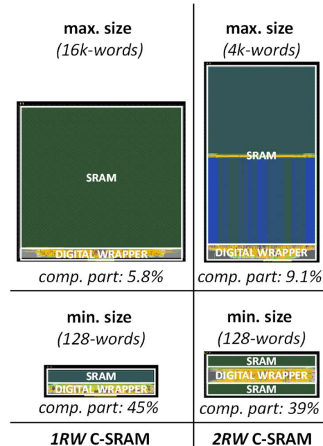
Figure 10 Floorplanning (post P&R) and computing part (%) of 1RW (left) and 2RW (right) C-SRAM macros for the minimum and maximum size allowed by the memory compilers selected.
